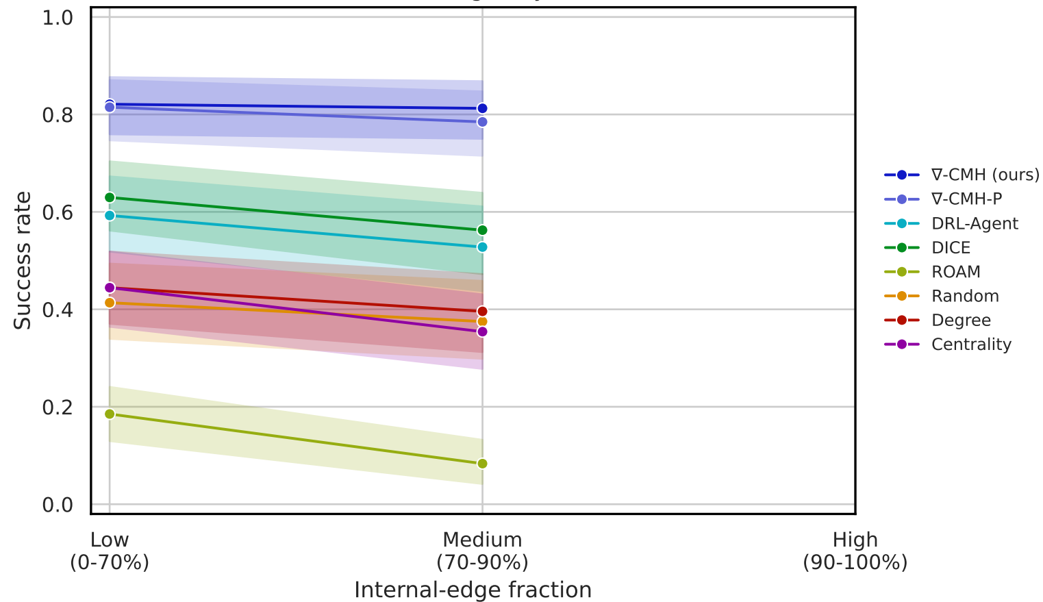
kar — greedy
