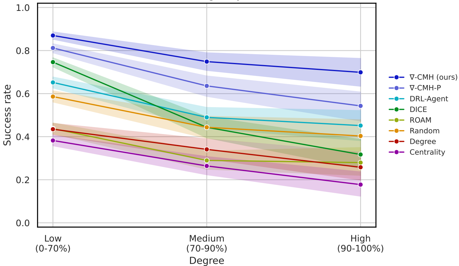
vote — greedy
