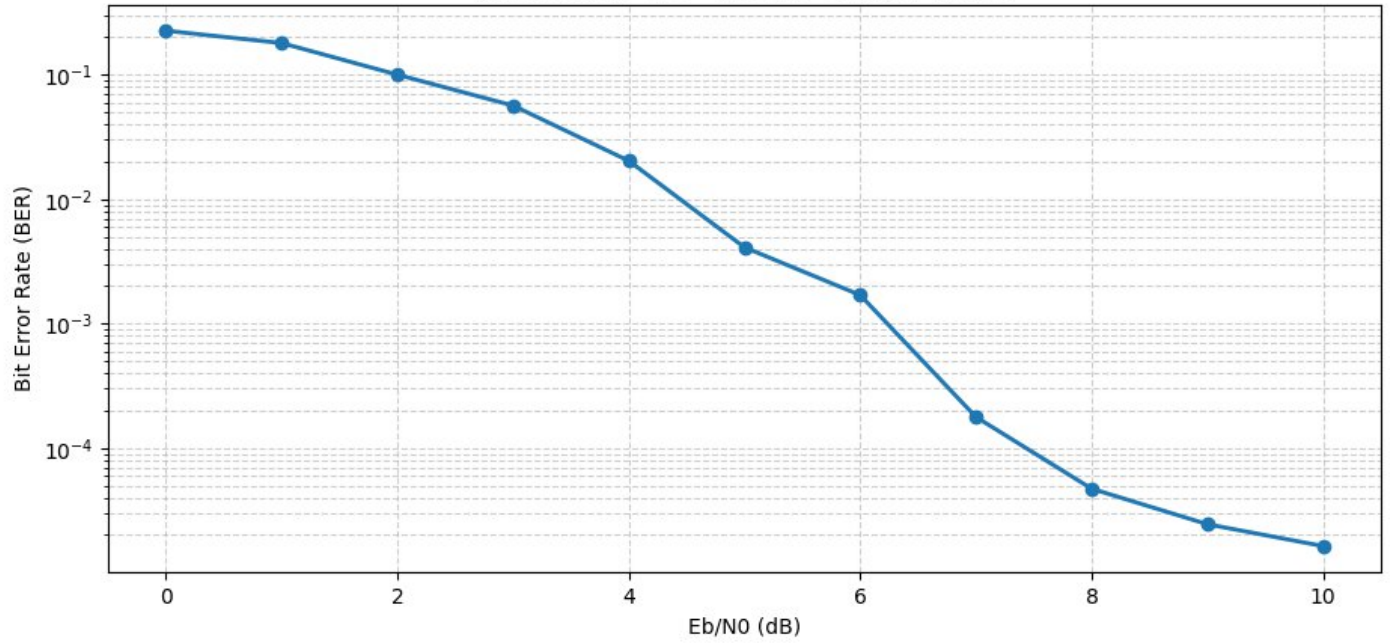
Conv. Encoded DS-CDMA over AWGN (Rate-1/2, K=3, G=(7,5), N=8, Hard Viterbi)
