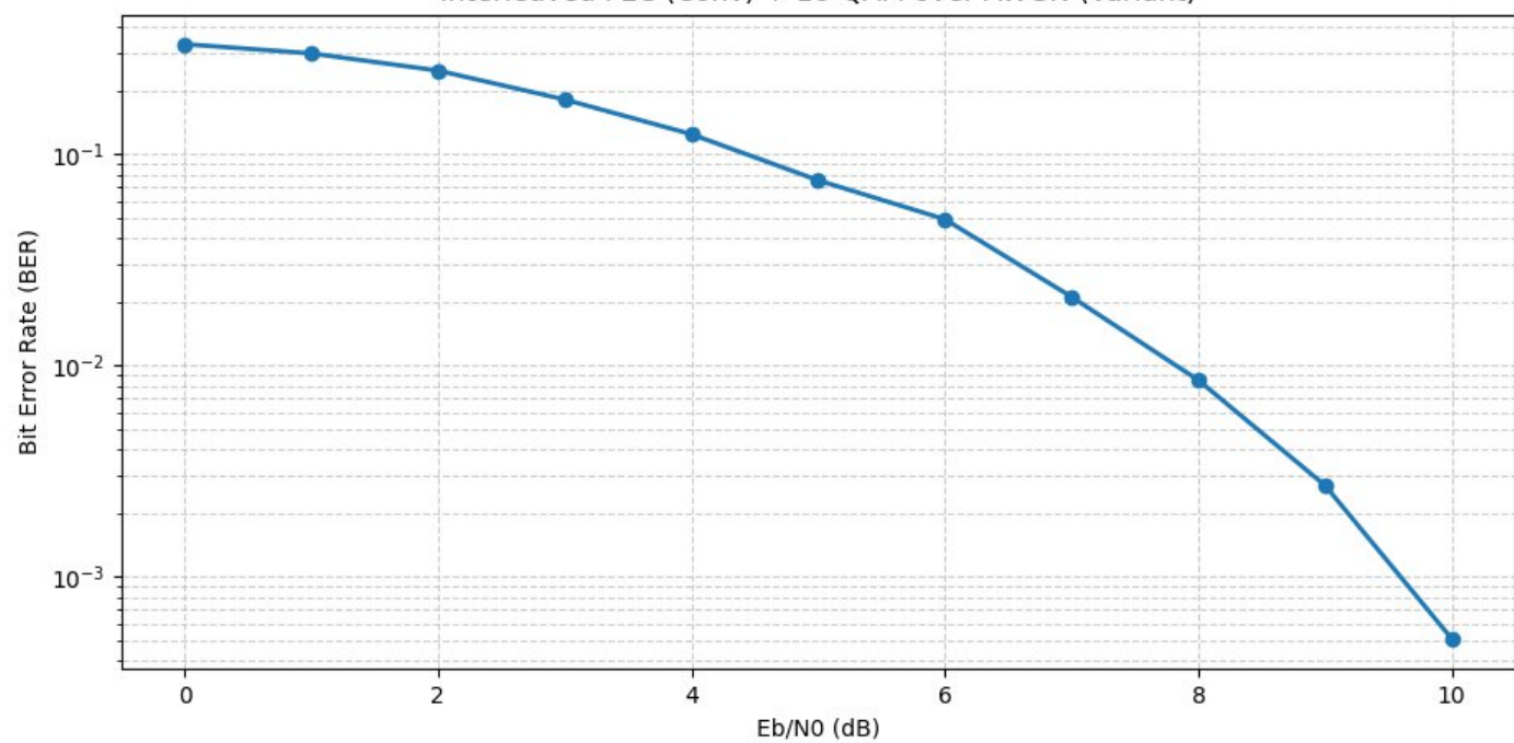
Interleaved FEC (Conv) + 16-QAM over AWGN (Variant)
