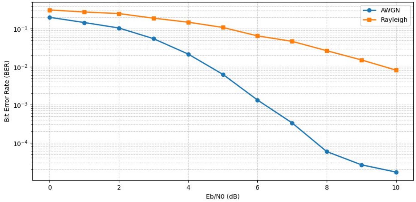
Conv-Coded DS-CDMA: AWGN vs Rayleigh (Variant)
