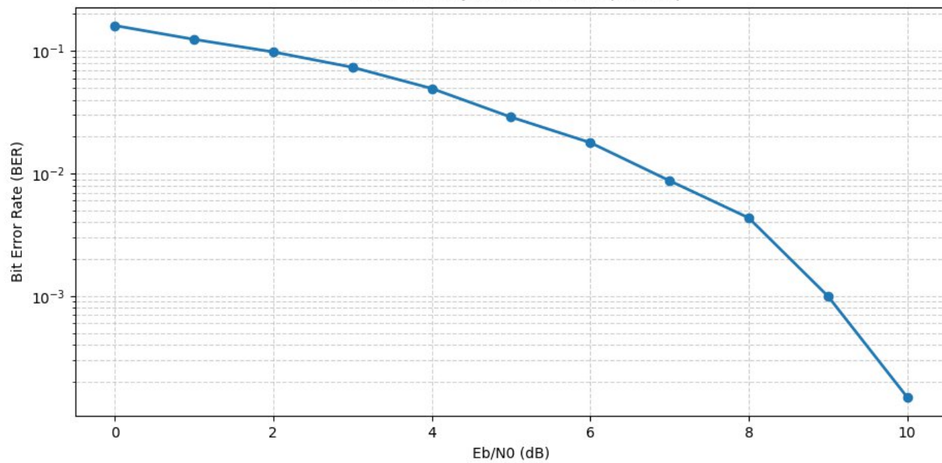
Differential OQPSK over AWGN (Variant)
