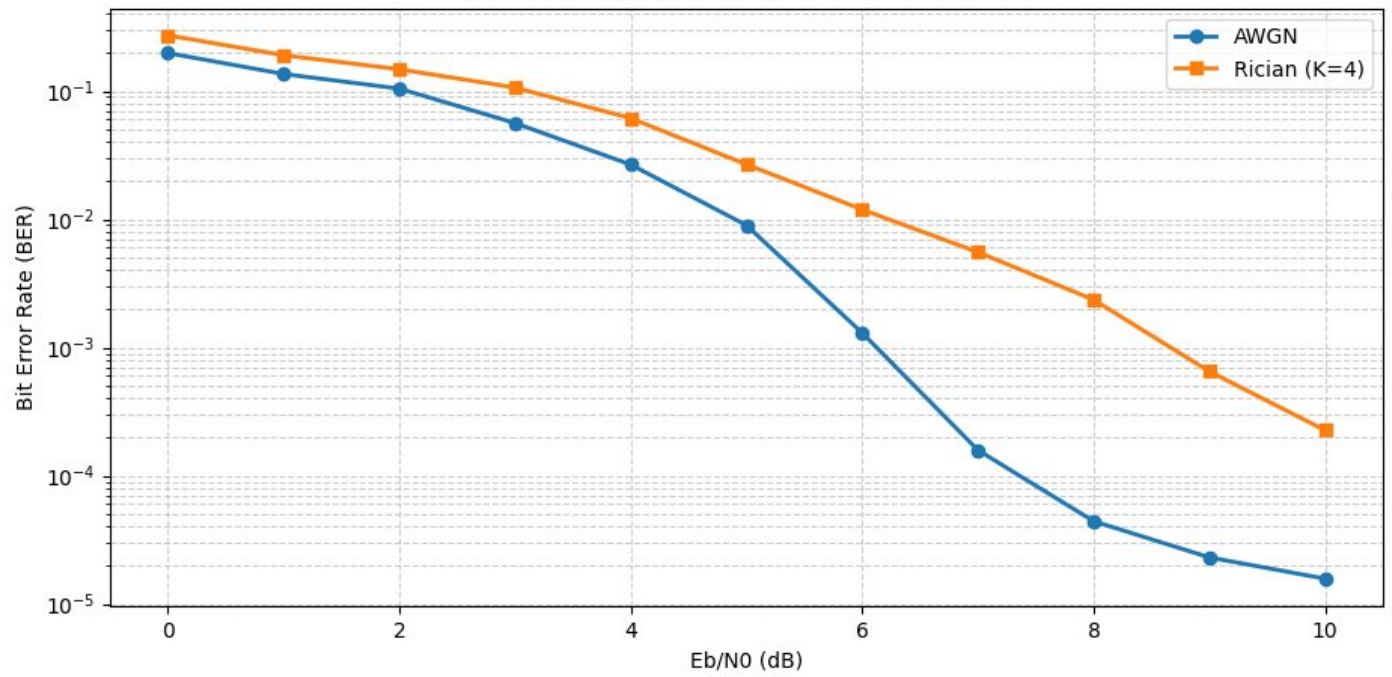
Conv-Coded DS-CDMA: AWGN vs Rician (Variant)
