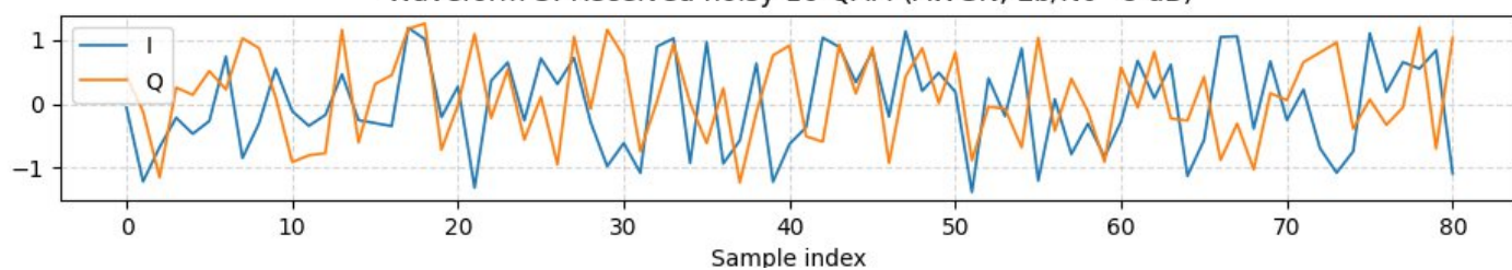
Waveform 3: Received noisy 16-QAM (AWGN, E_b/N_0=8 dB)
