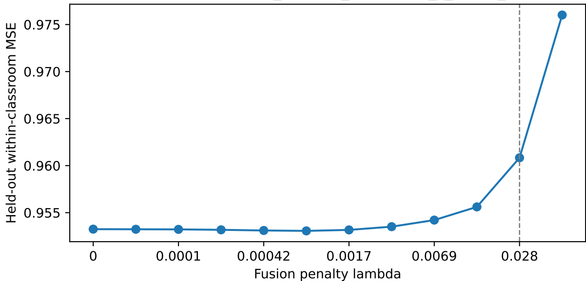
Penalty selection: 6plus_support_sensitivity_z_grade_primary
