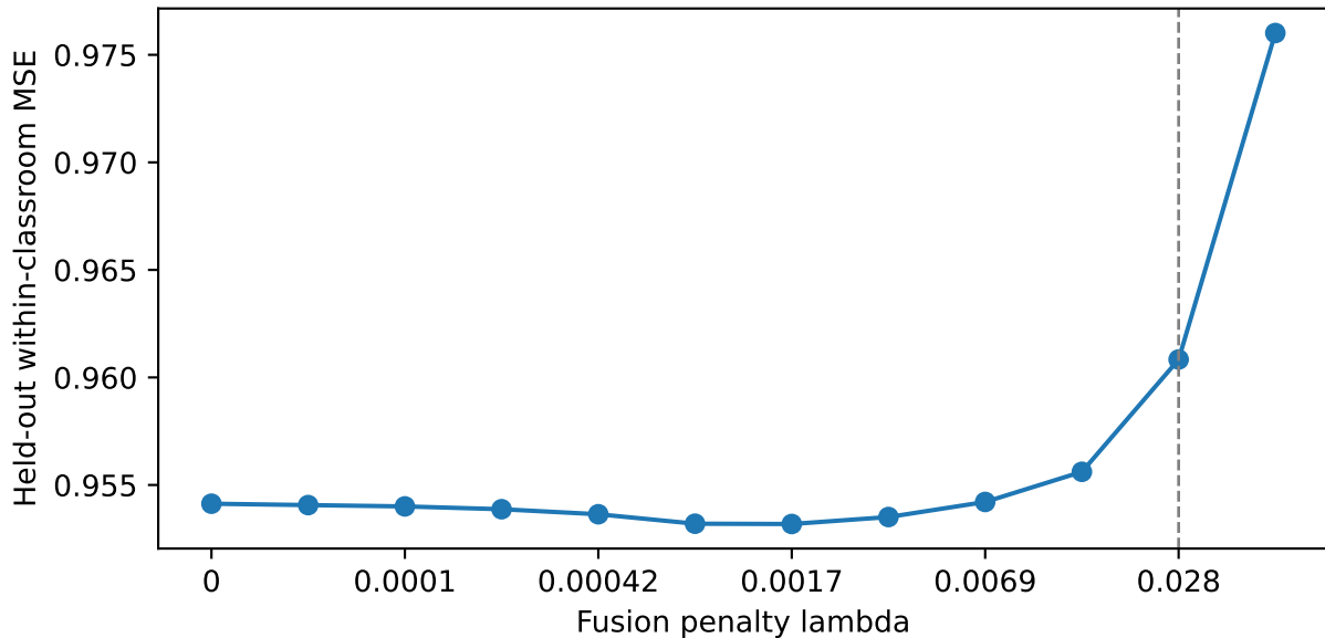
Penalty selection: 7plus_z_grade_primary
