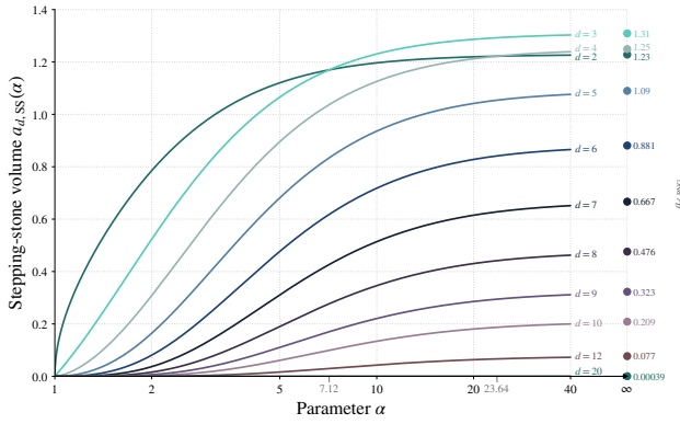
Figure 3: Numerical values of a_{d,SS}(\alpha) for several dimensions on a logarithmic \alpha -axis. The right endpoint shows a_{d,RNG} , the relative-neighborhood limit. The auxiliary labels 7.12 and 23.64 mark the two numerical intersections described in the text.
