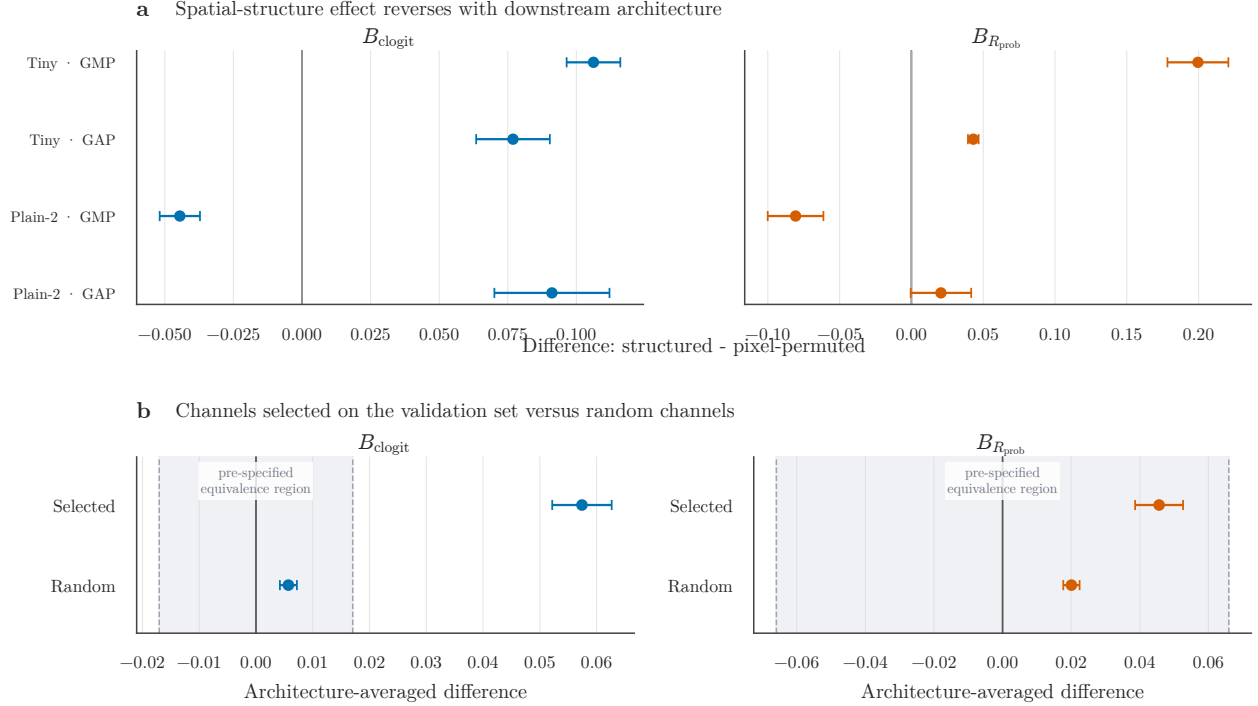
Figure 4: Pixel-permuted control experiment on independent renderer blocks. (a) Difference in B between the original structured bank and the pixel-permuted bank for channels selected on the validation set, shown separately for each architecture on two_concepts . The spatial effect reverses sign in plain2_w16_gmp . Bars are paired 95% t intervals over 100 renderer blocks. (b) Differences between the structured and pixel-permuted banks, averaged across architectures, for channels selected on the validation set and for random channel sets. Bars are 90% intervals used by the pre-specified TOST procedure; shaded regions denote the pre-specified equivalence margins, defined as 20% of the mean absolute B from the earlier architecture study. The centered-logit average for channels selected on the validation set is not equivalent, whereas the probability-error average for those channels and both random-channel averages fall within their respective pre-specified margins.
