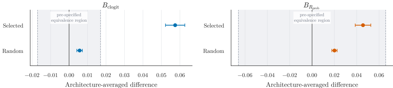
b Channels selected on the validation set versus random channels
