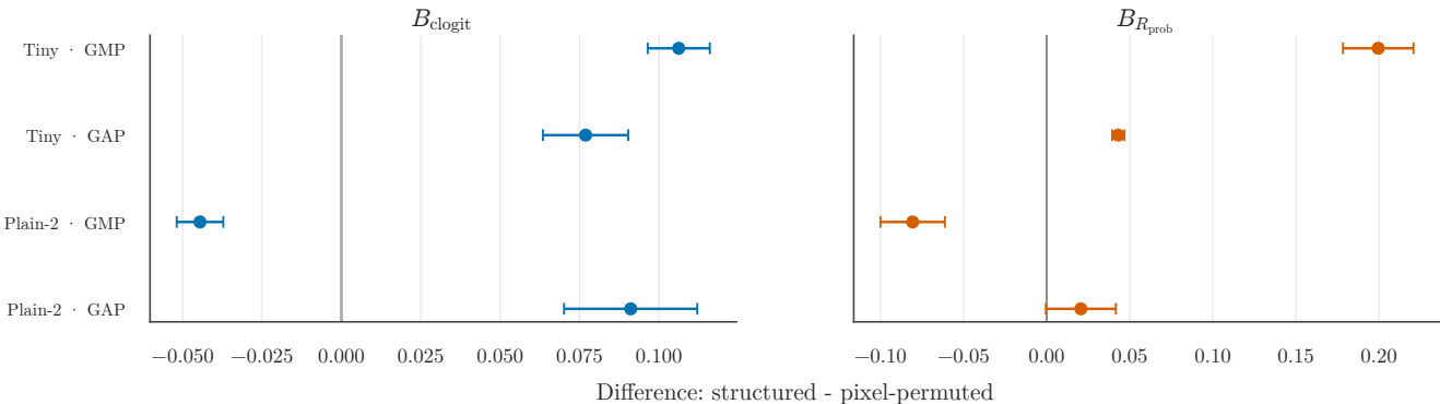
a Spatial-structure effect reverses with downstream architecture
