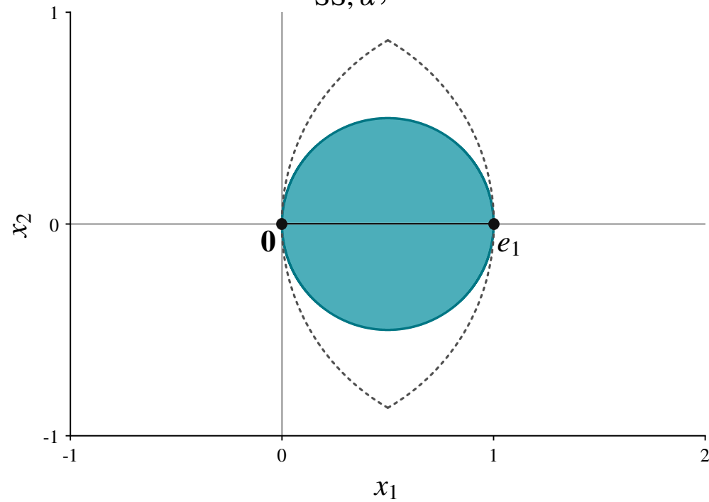
K_{SS,\alpha}, \alpha = 2
