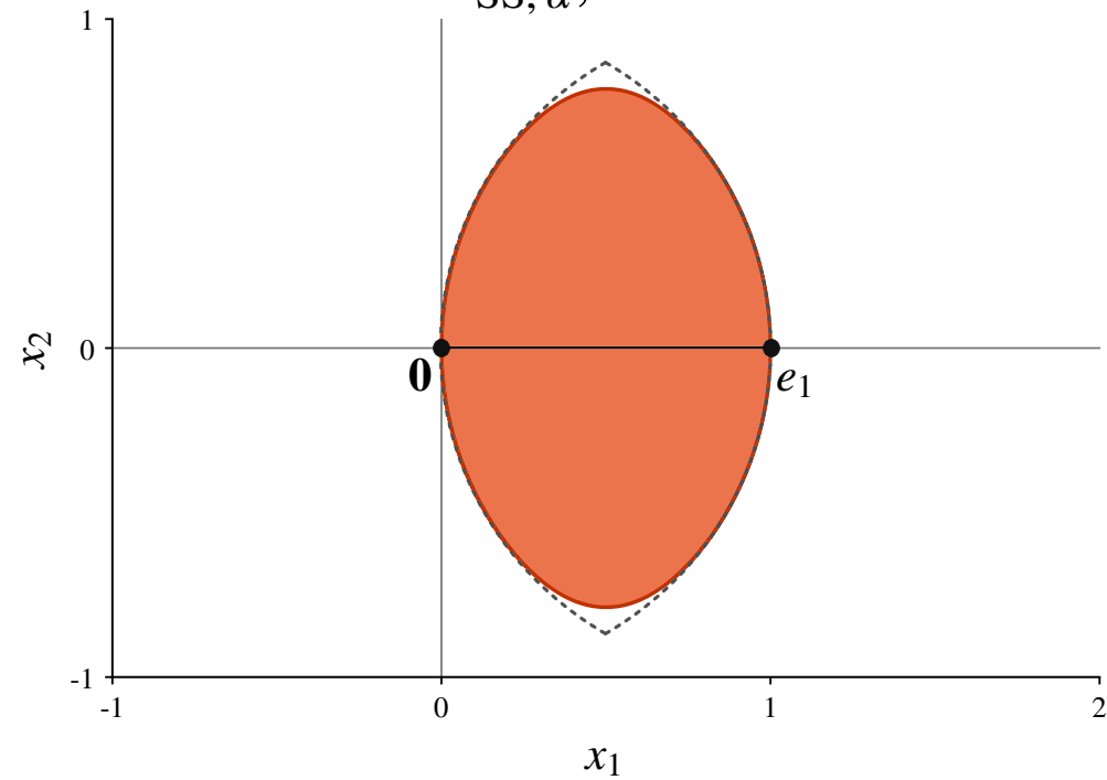
K_{SS,\alpha}, \alpha = 10
