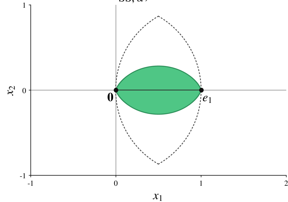
K_{SS,\alpha}, \alpha = 1.25
