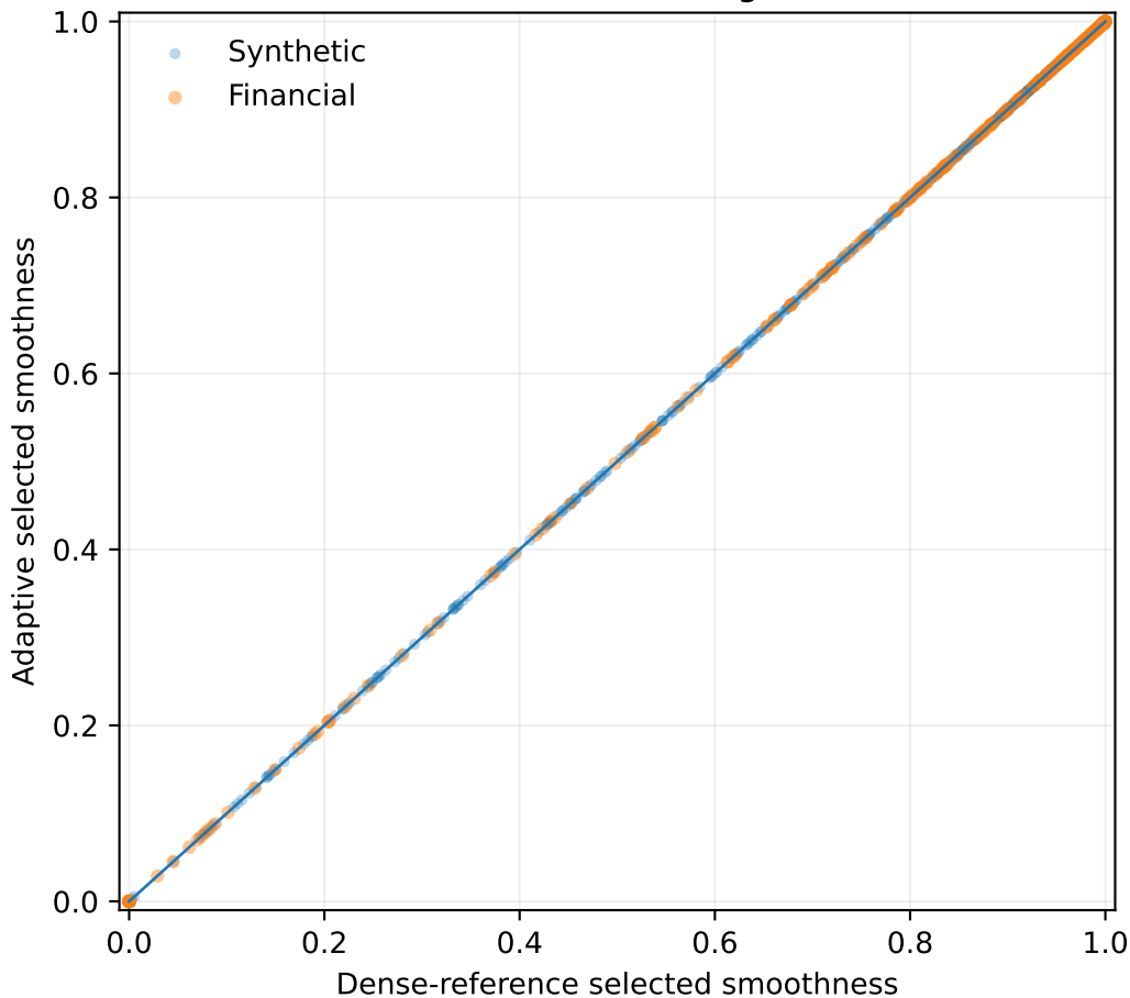
Selected-smoothness agreement
