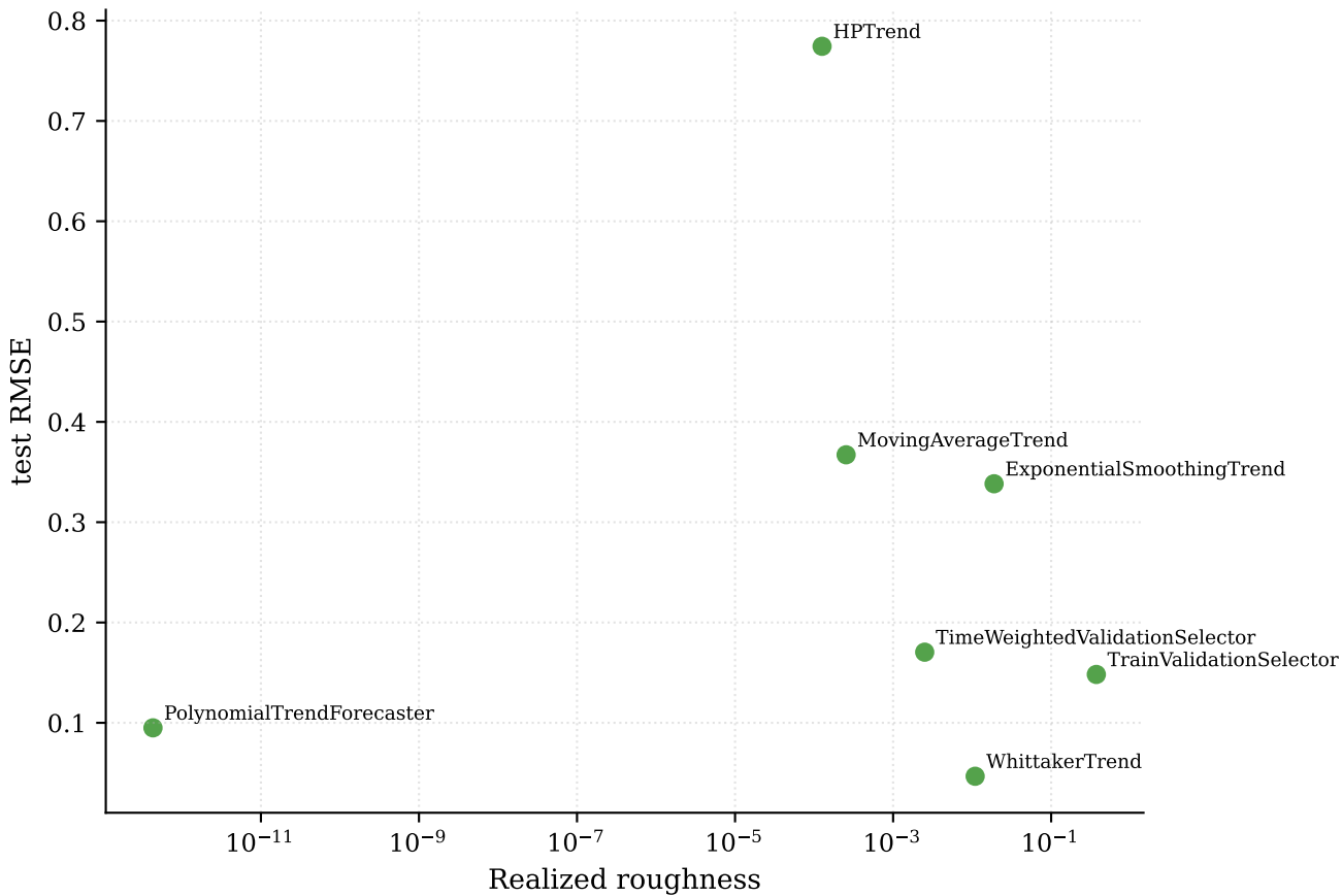
Realized roughness against test RMSE
