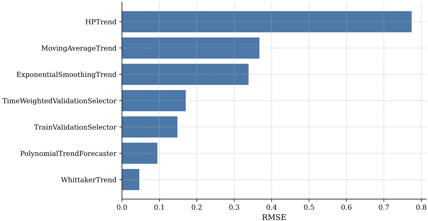
Test RMSE by method
