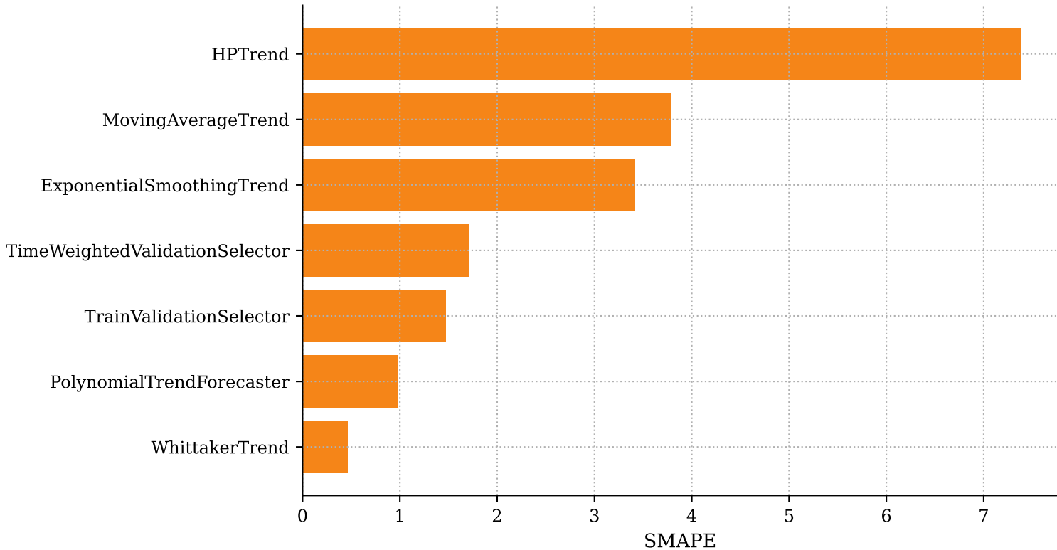
Test SMAPE by method
