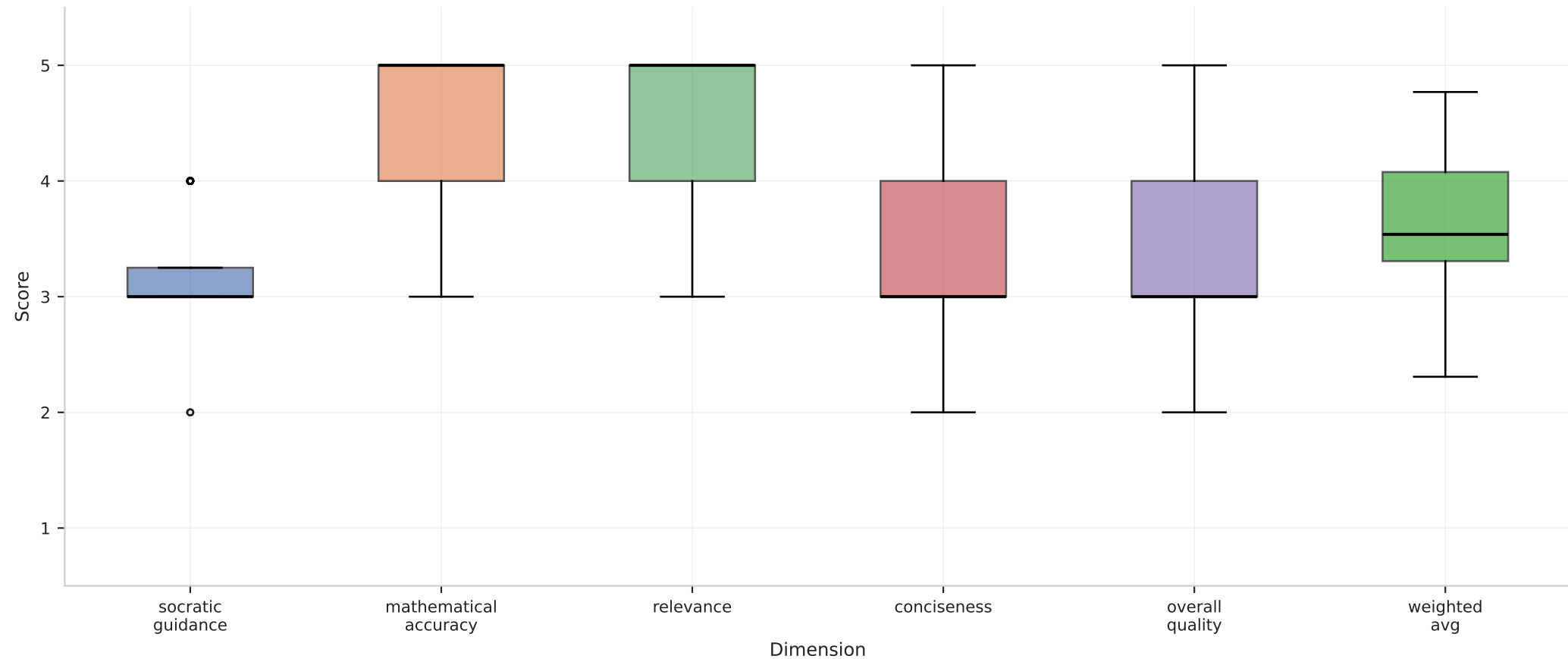
Score Distribution — Box & Whisker (with outliers)
