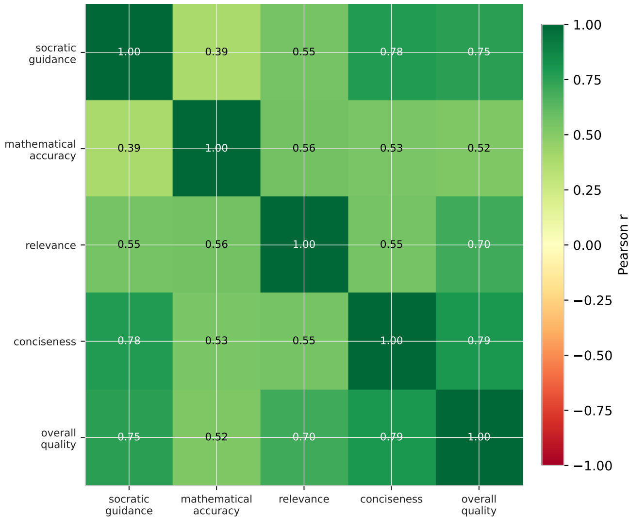
Cross-Dimension Pearson Correlation Matrix
