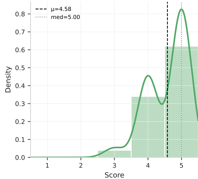
Relevance
