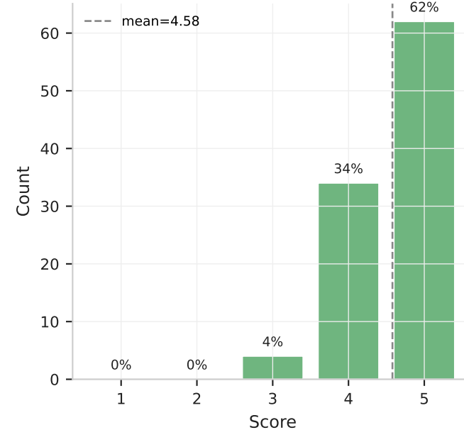
Relevance
