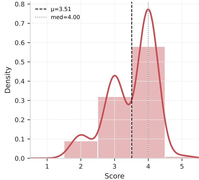
Conciseness
