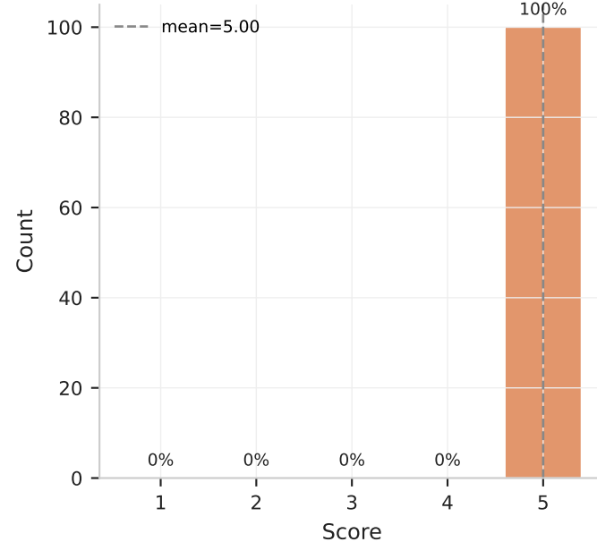
Mathematical Accuracy
