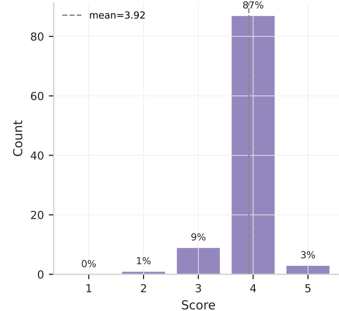
Overall Quality
