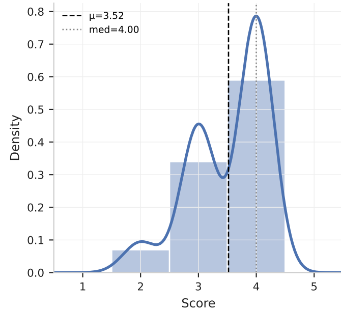
Socratic Guidance
