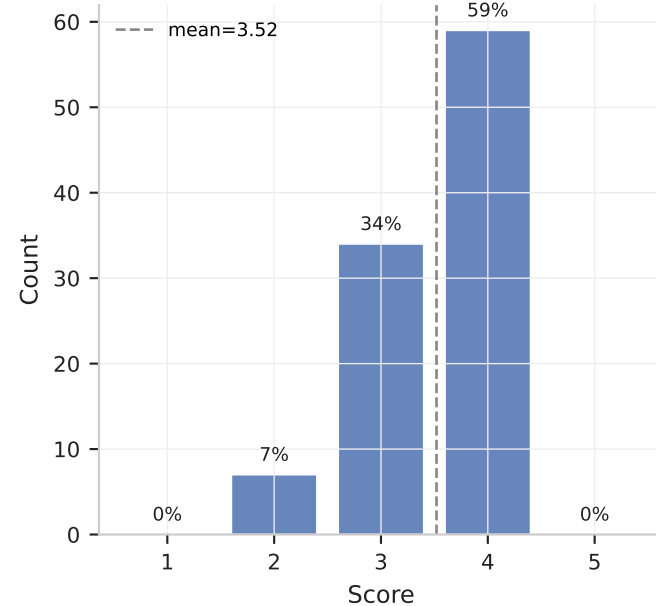
Socratic Guidance
