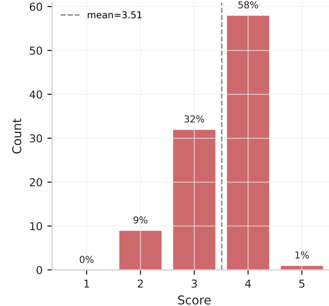
Conciseness
