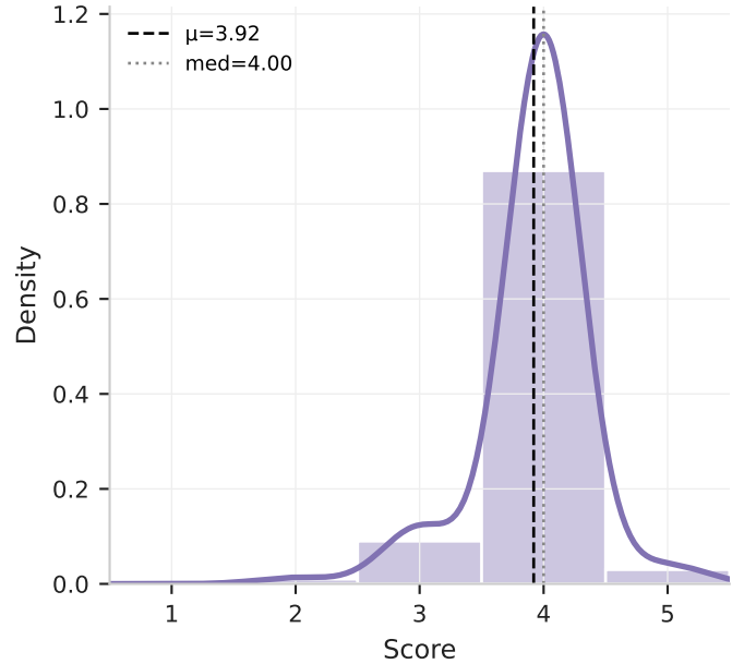
Overall Quality
