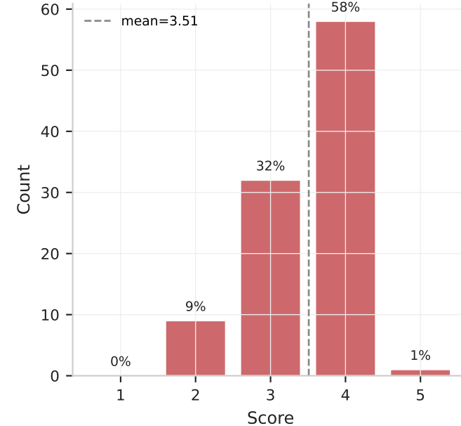
Conciseness
