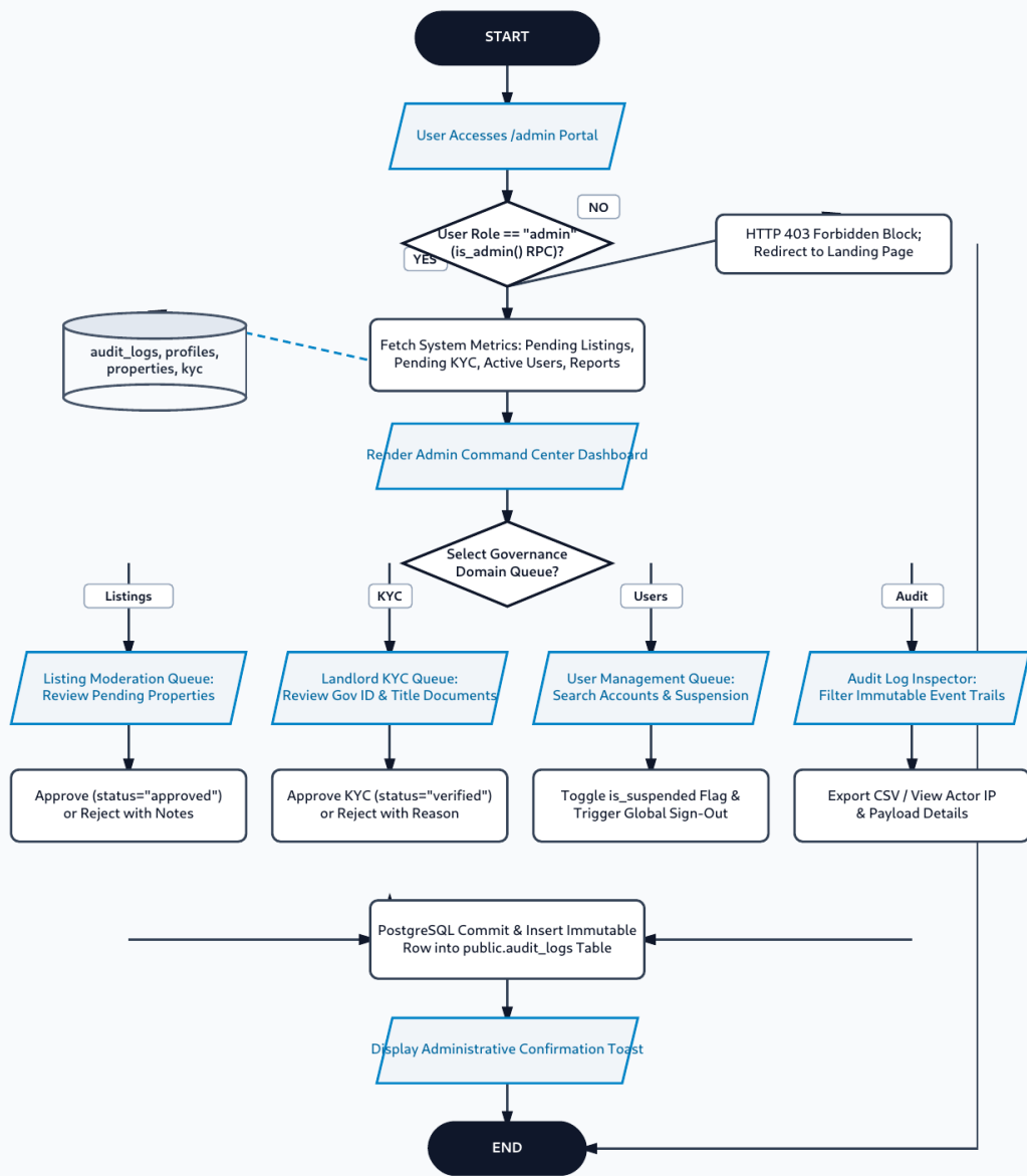
AbangCebu AI: Administrative Moderation & Governance Flowchart
