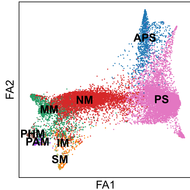
cell_type_abbr
