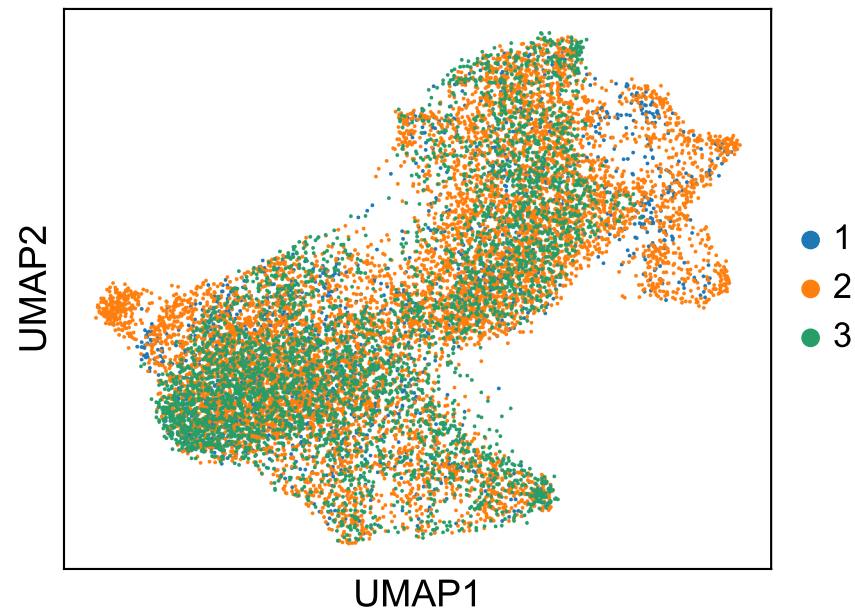
batch
