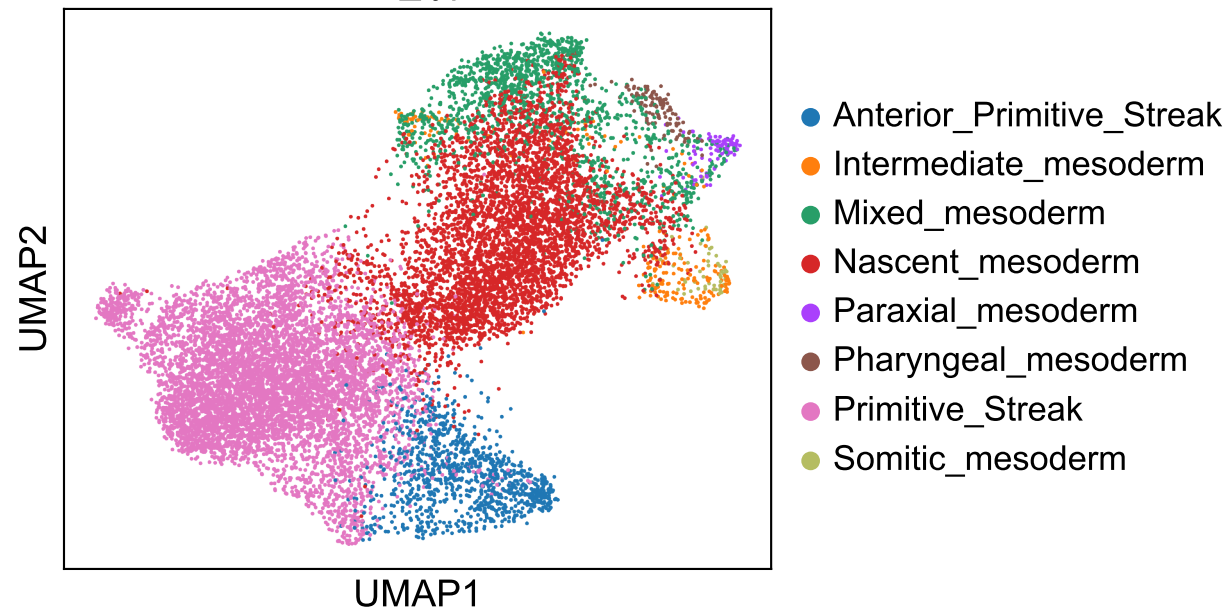
cell_type
