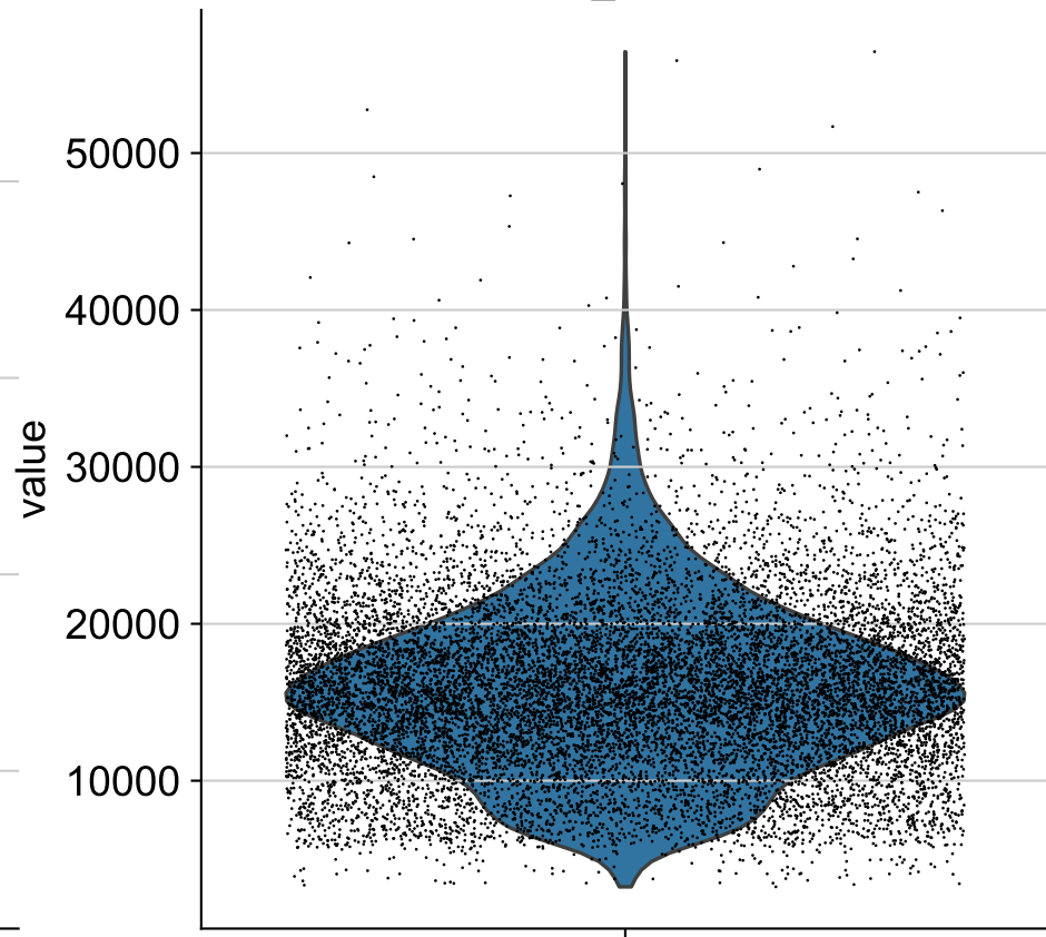
total_counts
