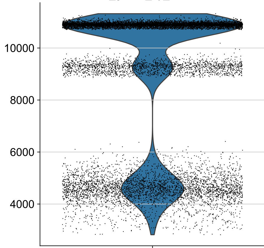
n_genes_by_counts
