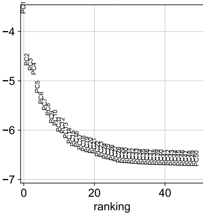
variance ratio
