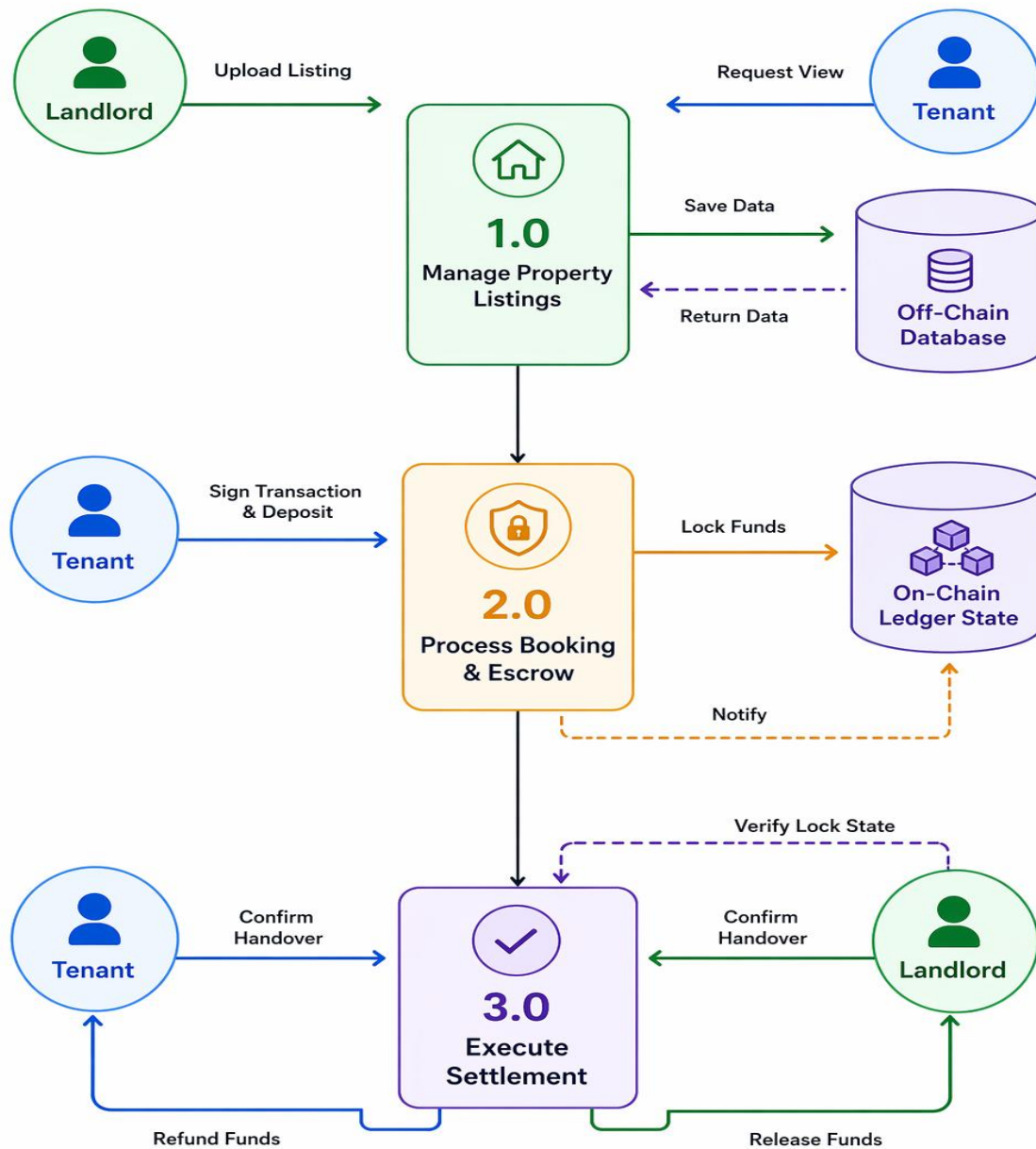
Figure 9: The Level 1 data flow diagram
