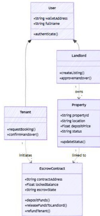
Figure 6: A class diagram defines the static structure of the system
