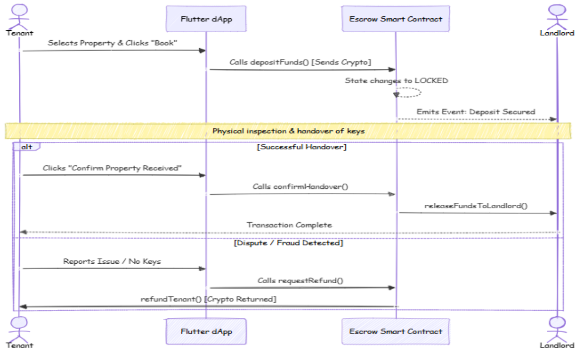
Figure 7: A sequence diagram maps the dynamic, chronological workflow of the system
