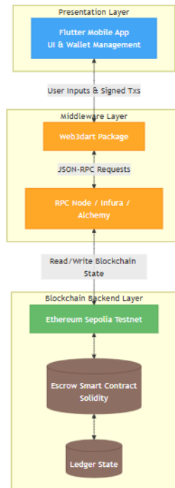
Figure 2: Preliminary System Architecture
