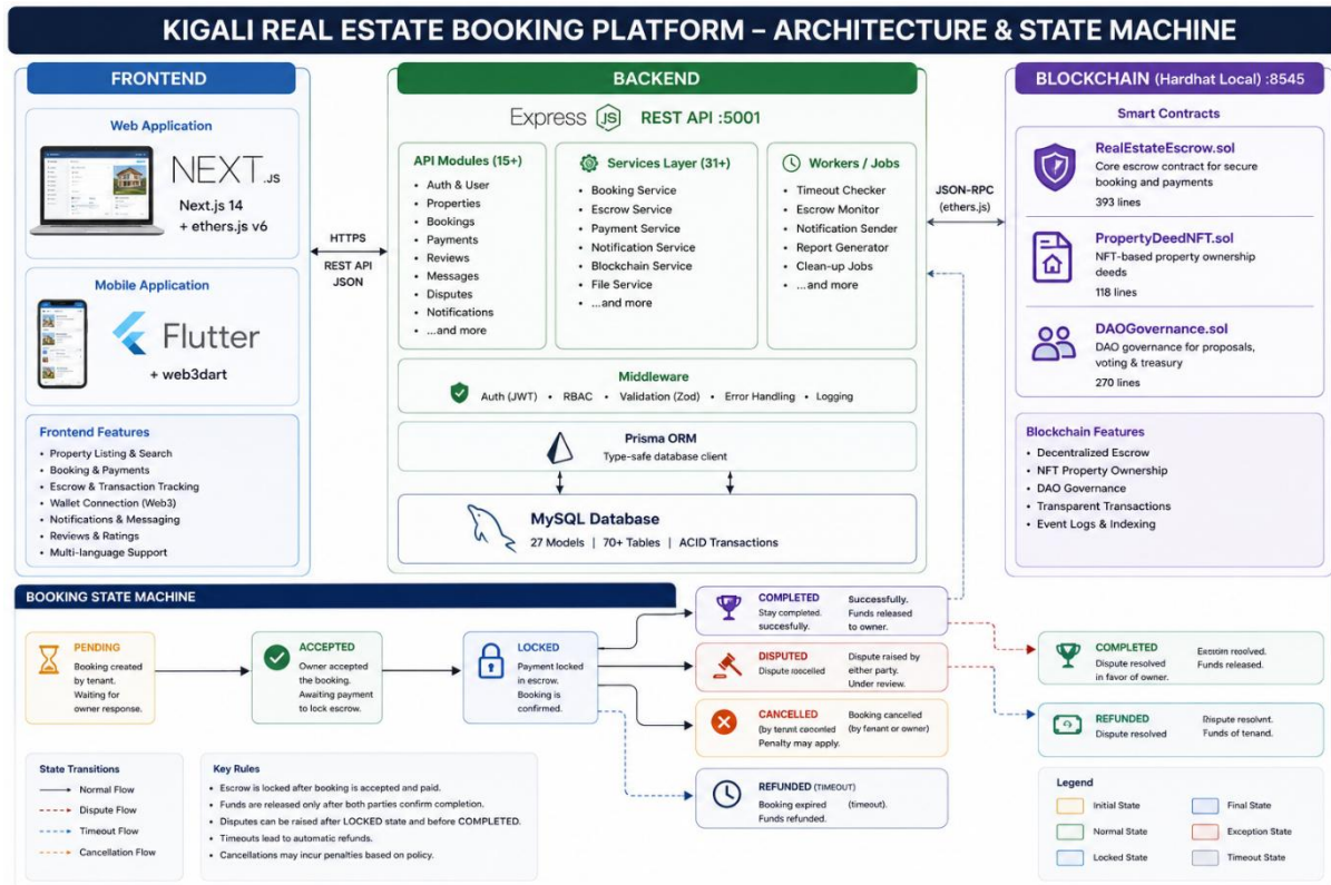
Figure 23: KIGALI REAL ESTATE BOOKING PLATFORM - ARCHITECTURE & STATE MACHINE
