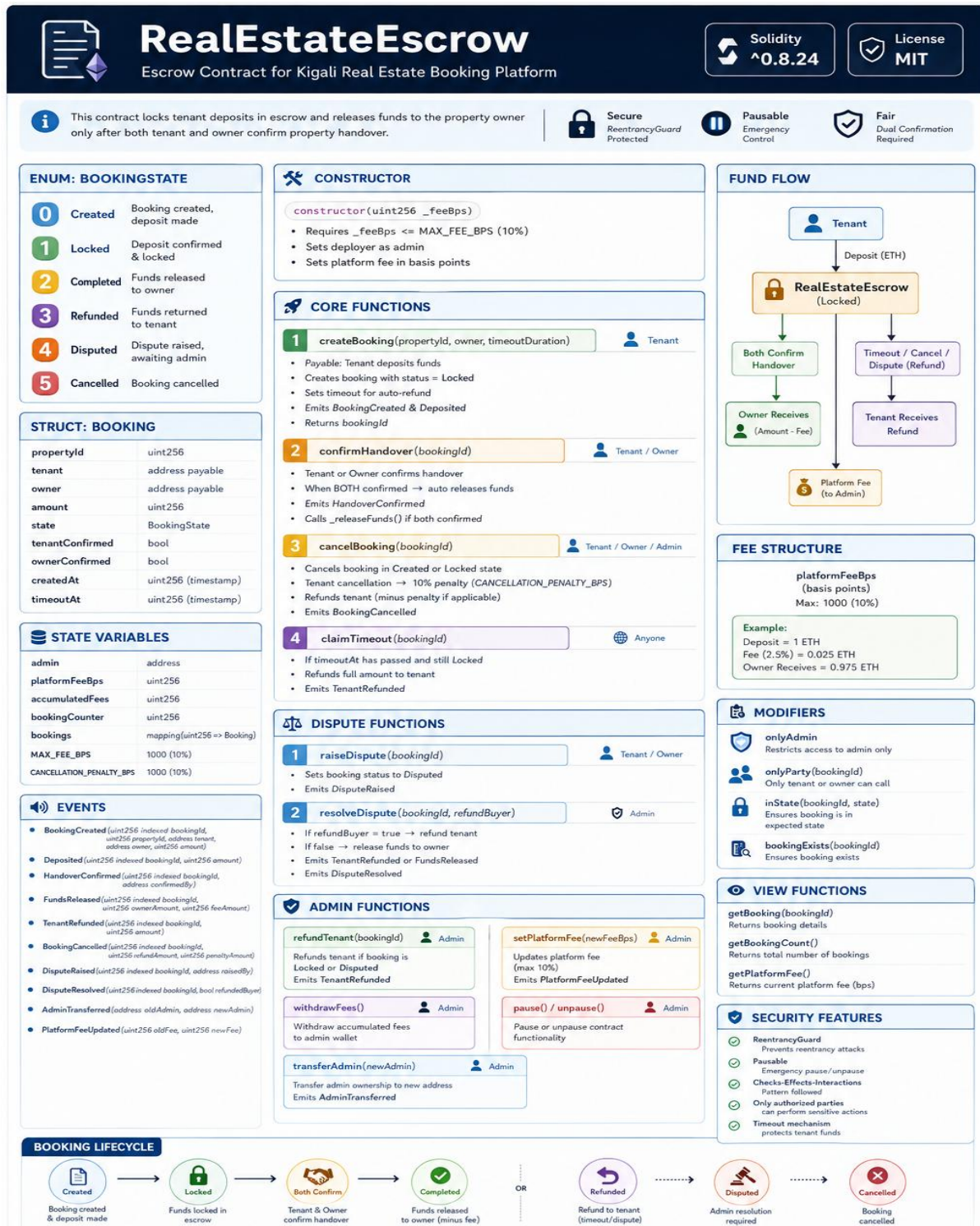
Figure 21: RealEstateEscrow Escrow Contract for Kigali Real Estate Booking Platform
