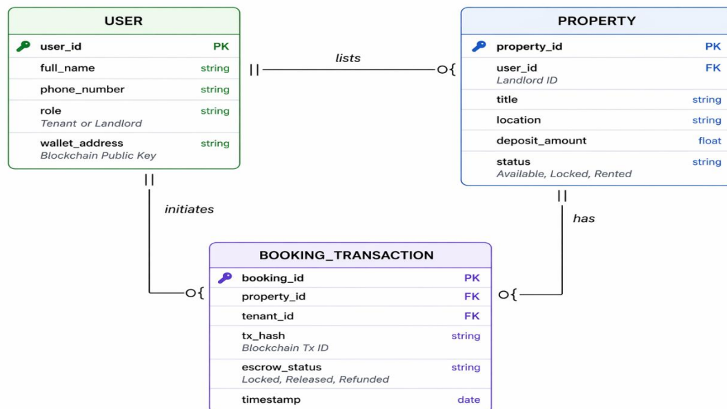
Figure 12: Entity Relationship Diagram (ERD)
