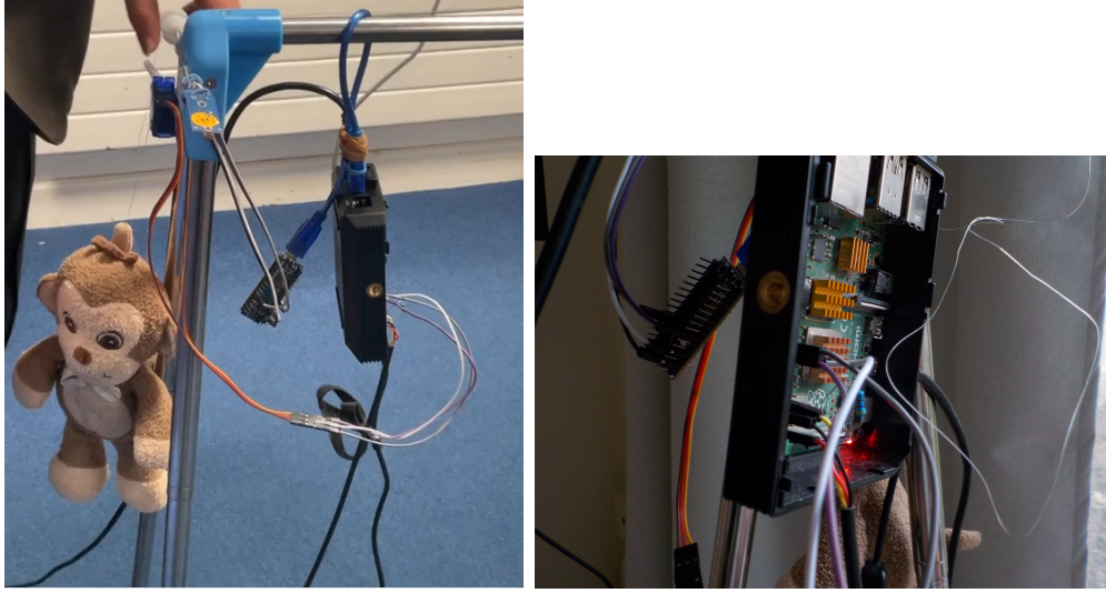
(a) Release System: Servo, pulley (b) Wiring on the RPi: Servo and temperature sensor are connected to the bracket. Raspberry Pi and Arduino GPIO pins, servo wired in grey, purple and white, temperature sensor wires in the rail. The temperature sensor (out red, black and yellow. In the background, of frame) is connected via the black the Arduino Nano has the light sensor cable pointing downwards. The mon-board connected to read data and provide power.
