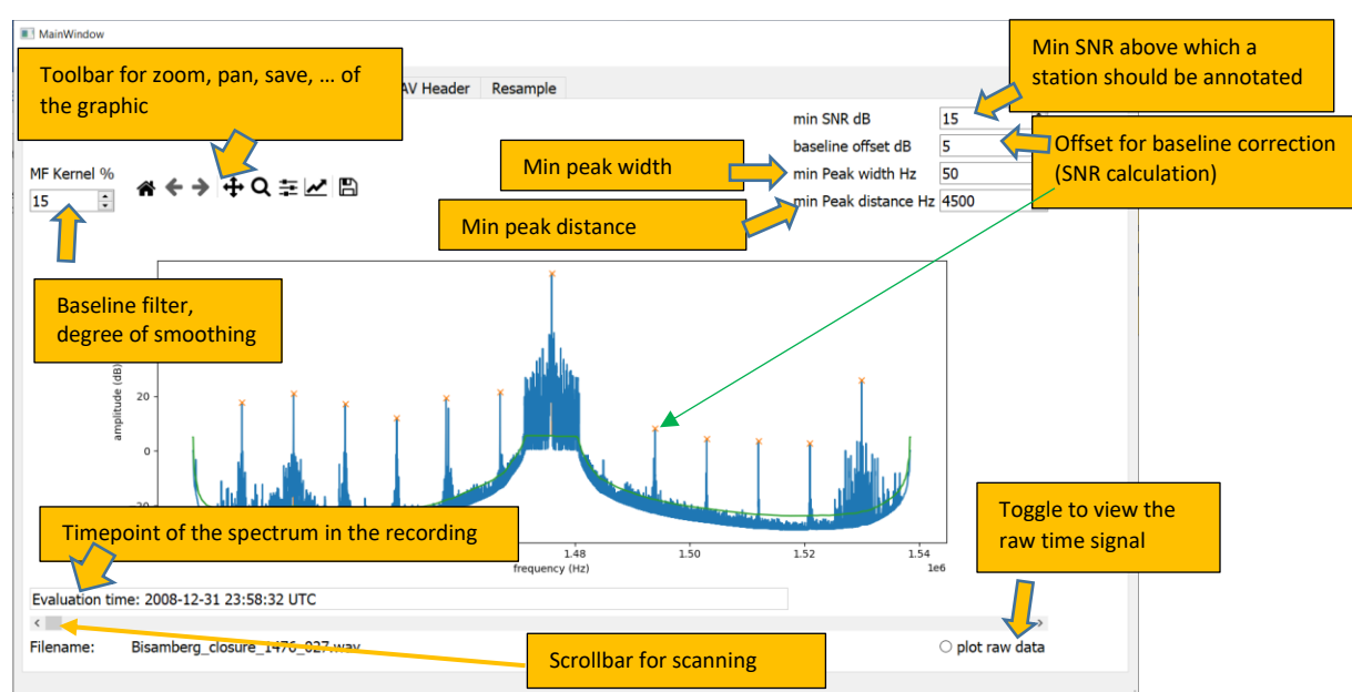
Fig. 1-11: Viewing the spectrum of a recording.
