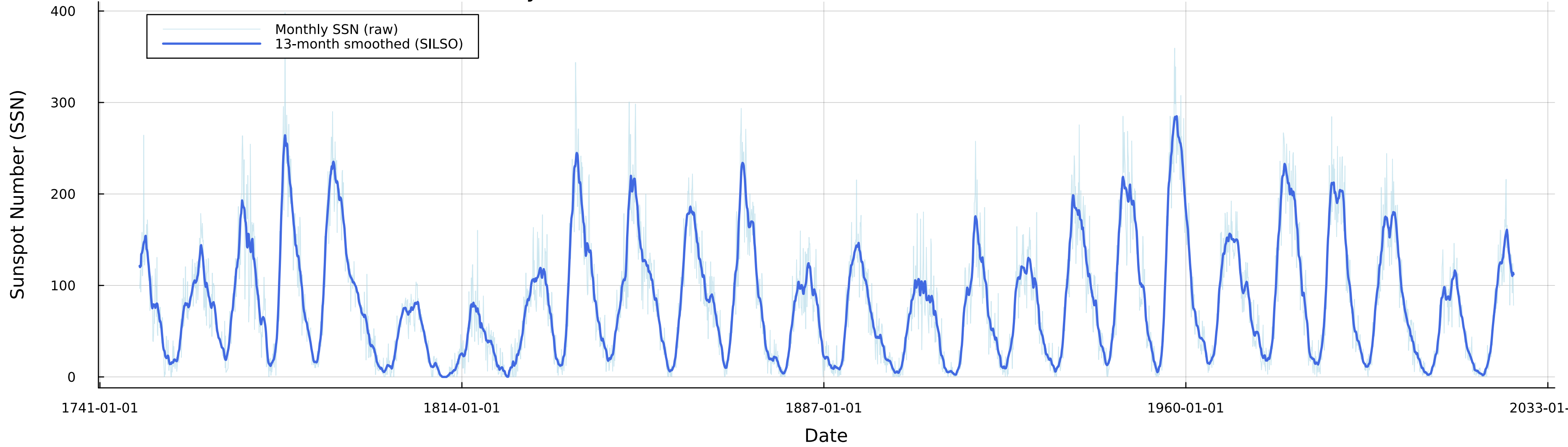
Monthly SSN and 13-Month Smoothed Series (SILSO, 1749-2026)
