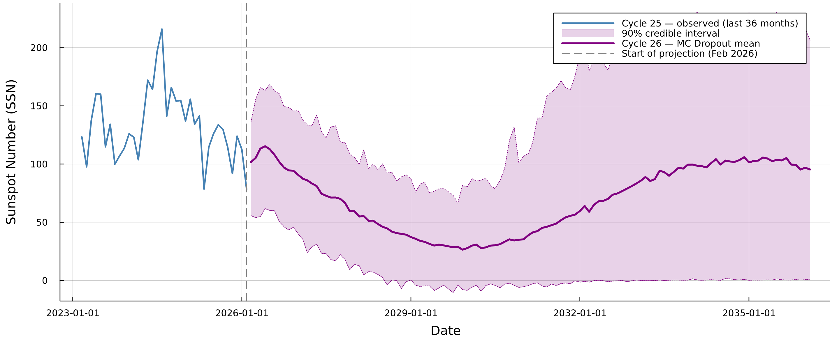
Solar Cycle 26 Projection — MC Dropout 90% Credible Interval (post-hoc, p=0.10 , N=200 stochastic passes; Gal & Ghahramani 2016)
