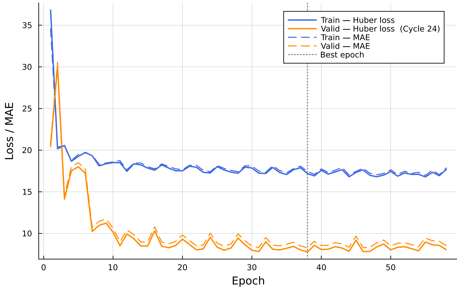
Training Curves (best epoch: 38)
