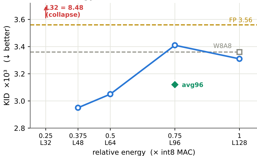
KID vs energy
