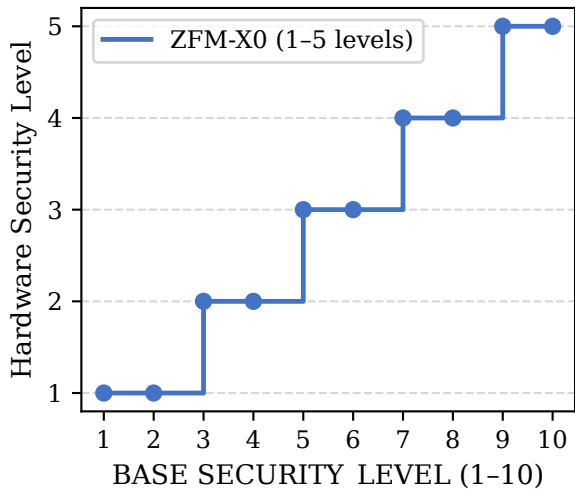
(a) Security Level Mapping
