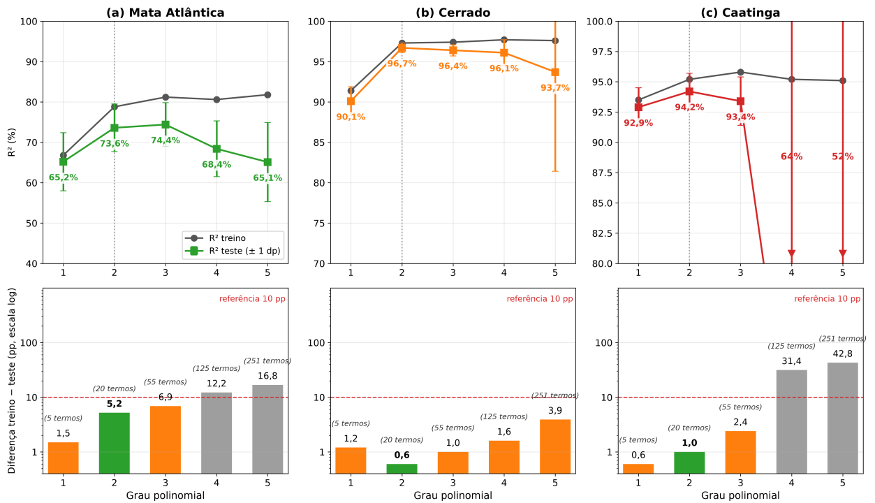
Figure 4: Selection of the polynomial degree of the MPRM-N in the three biomes: training and test R^2 and train-test gap by degree (RepeatedKFold 5 \times 30 ).
