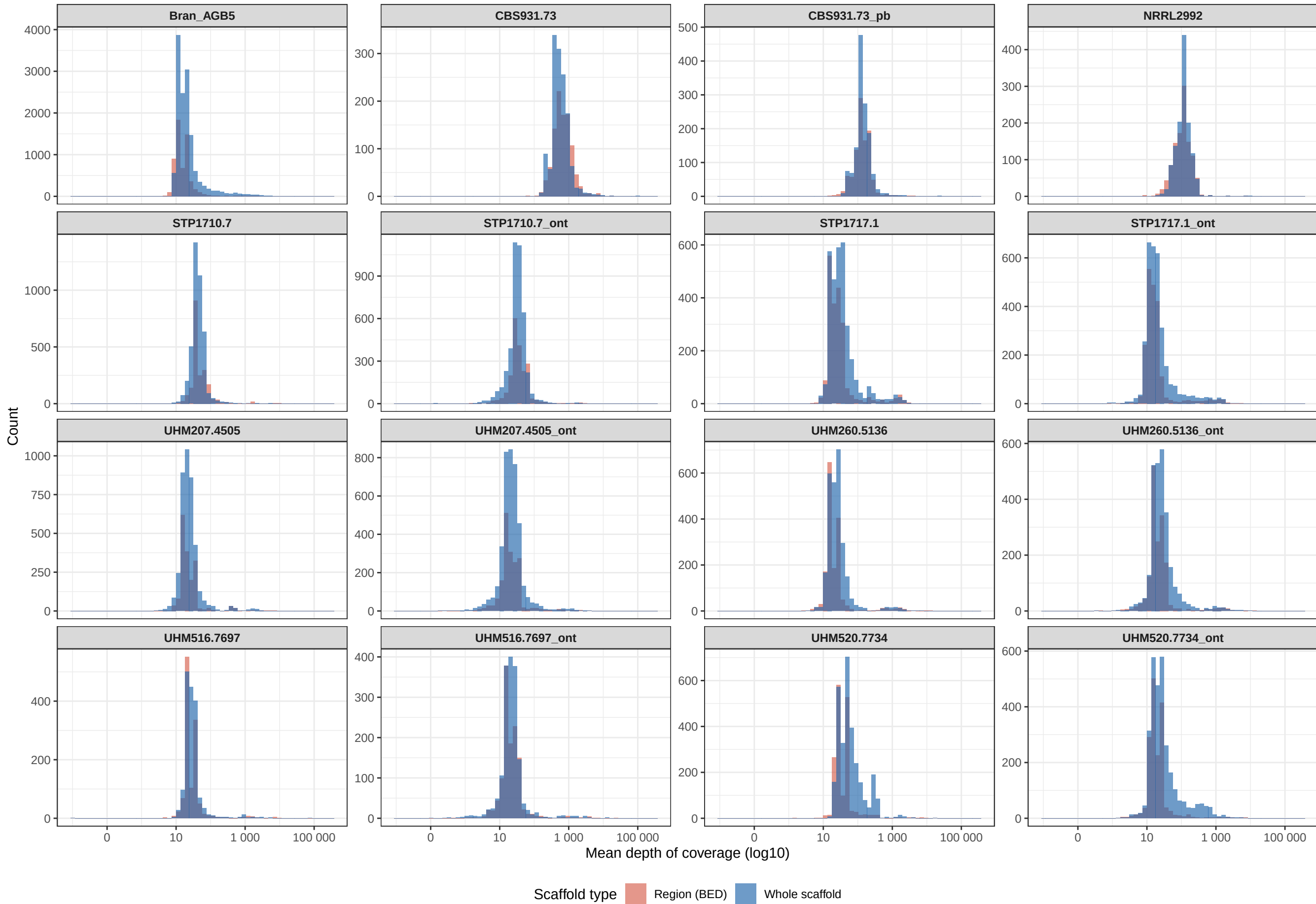
Distribution of per-scaffold mean coverage depth by strain (log10 scale)
