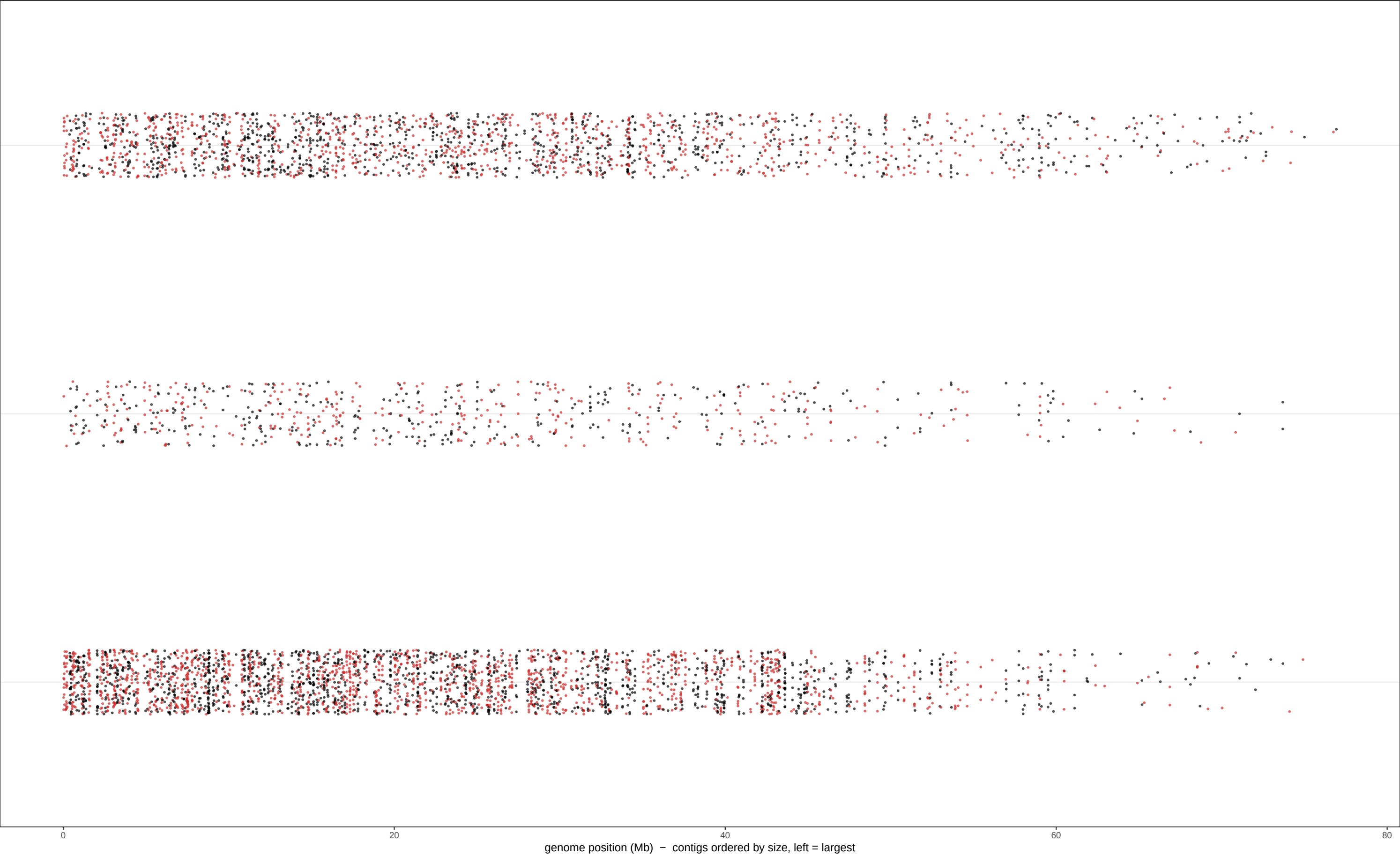
UHM516.7697 – genome-wide per-gene ploidy (Manhattan) alternating black/red marks consecutive contigs; winner = smallest delta-log-likelihood
