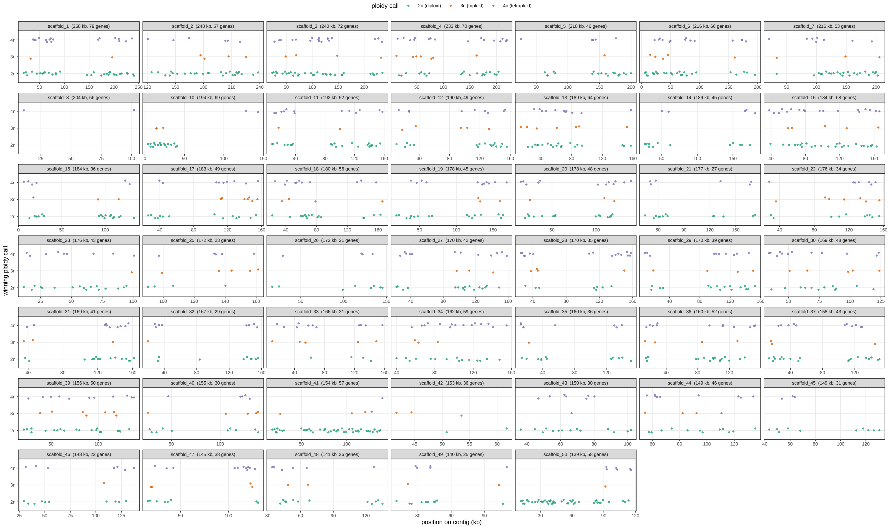
UHM516.7697 – per-gene ploidy, top 50 contigs by size winner = smallest delta-log-likelihood among d_dip/d_tri/d_tet (0/nan = missing, omitted)
