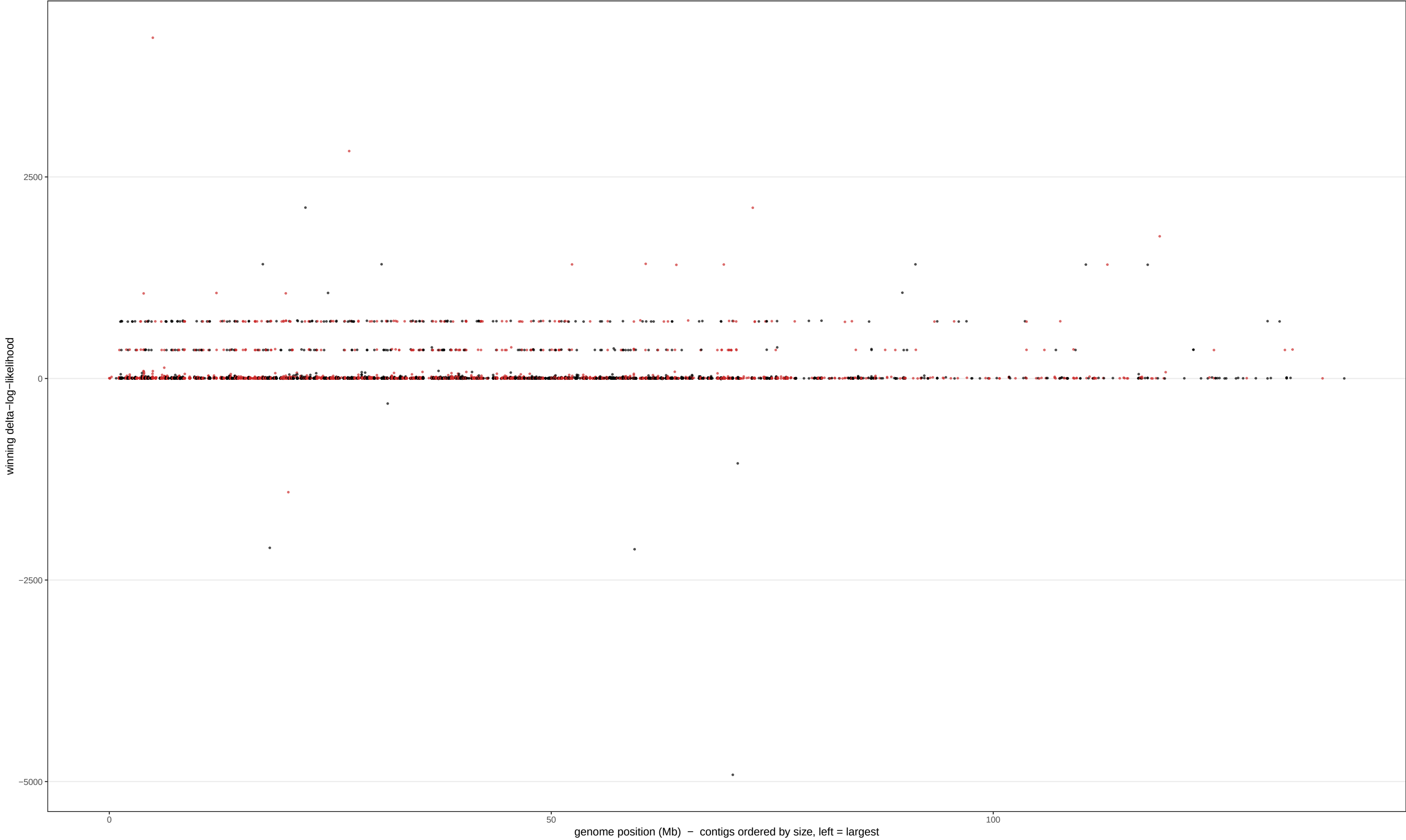
STP1710.7 – genome-wide per-gene ploidy (Manhattan) alternating black/red marks consecutive contigs; winner = smallest delta-log-likelihood
