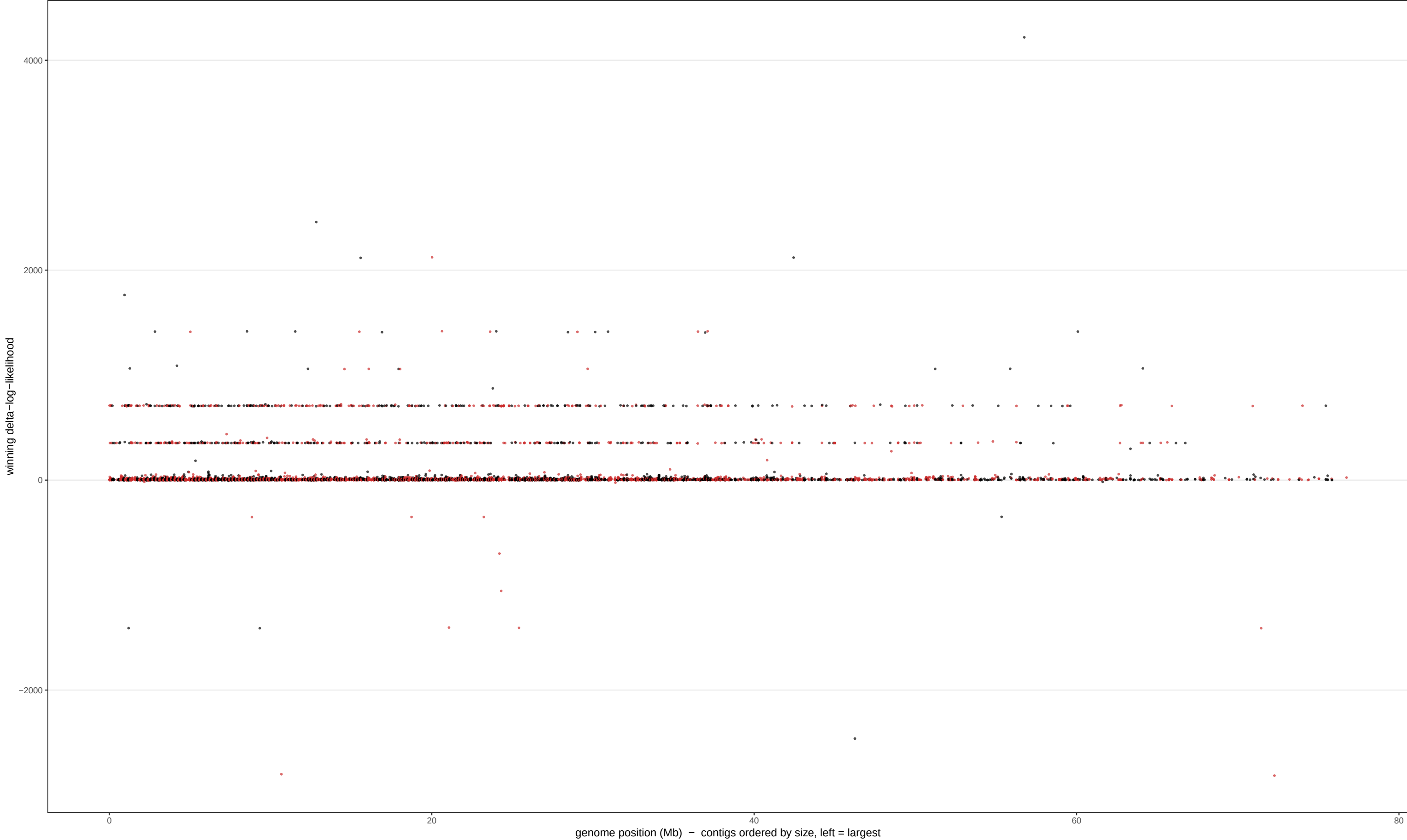
UHM520.7734 – genome-wide per-gene ploidy (Manhattan) alternating black/red marks consecutive contigs; winner = smallest delta-log-likelihood
