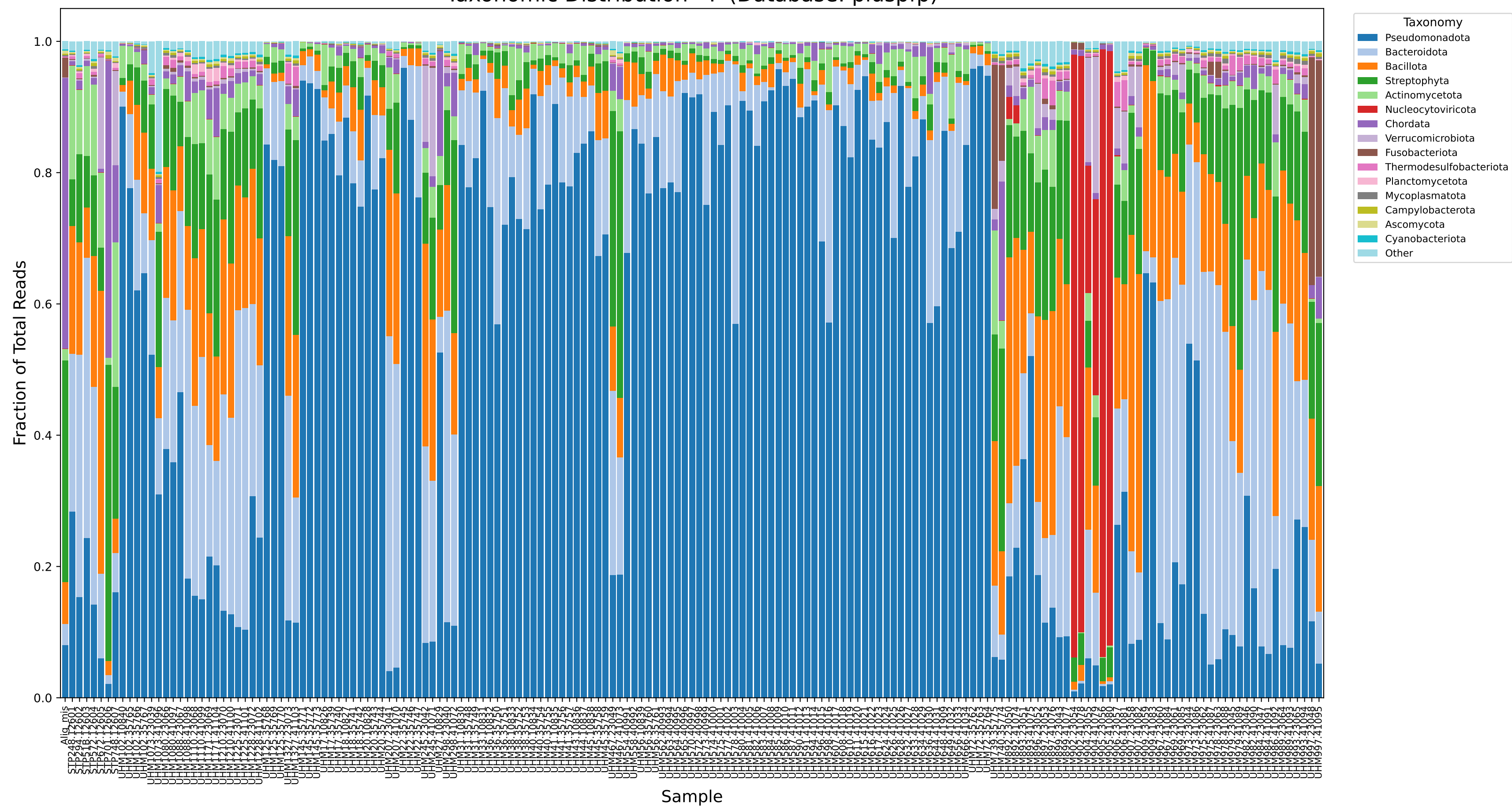
Taxonomic Distribution - P (Database: pluspfp)
