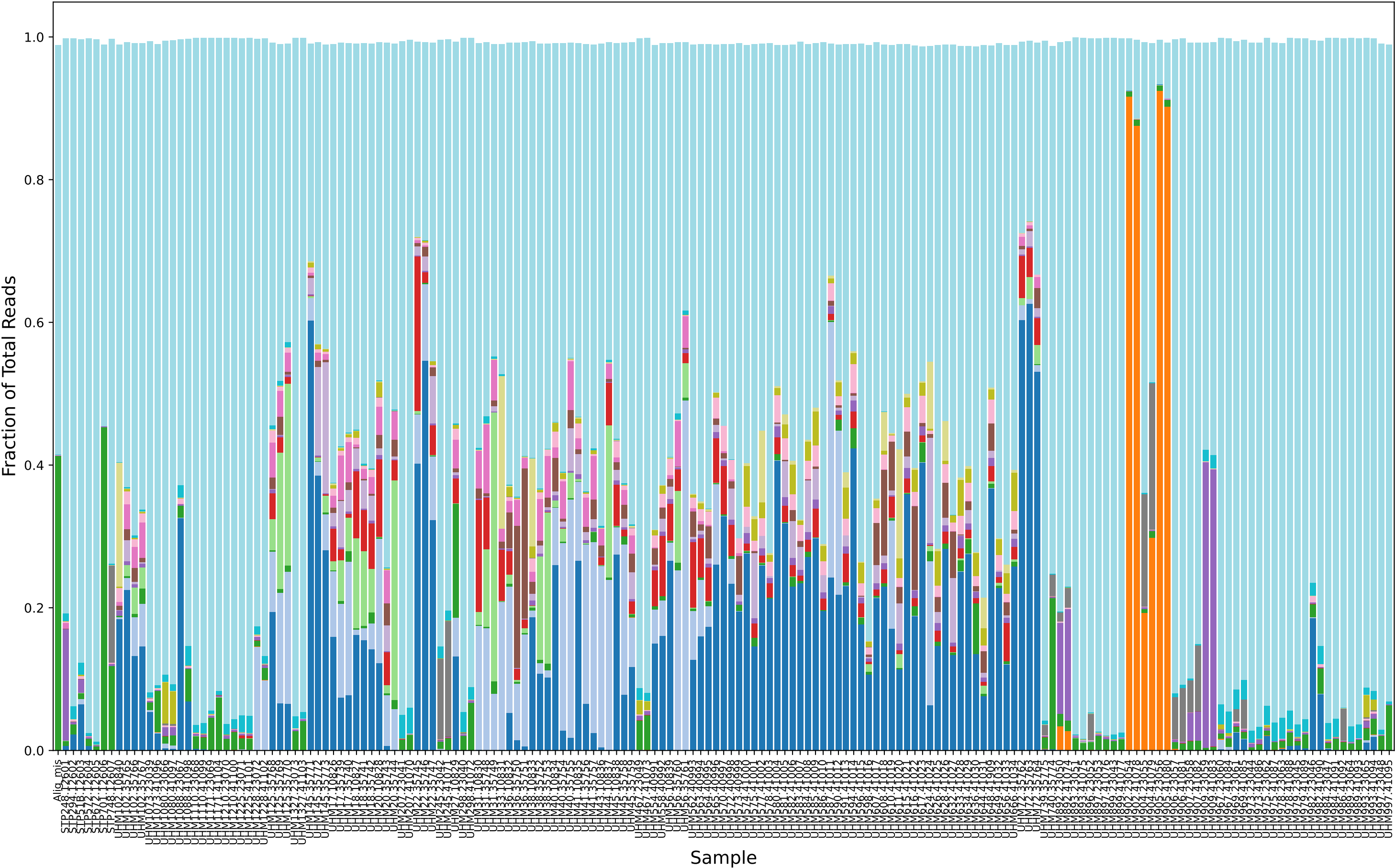
Taxonomic Distribution - S (Database: pluspfp)
