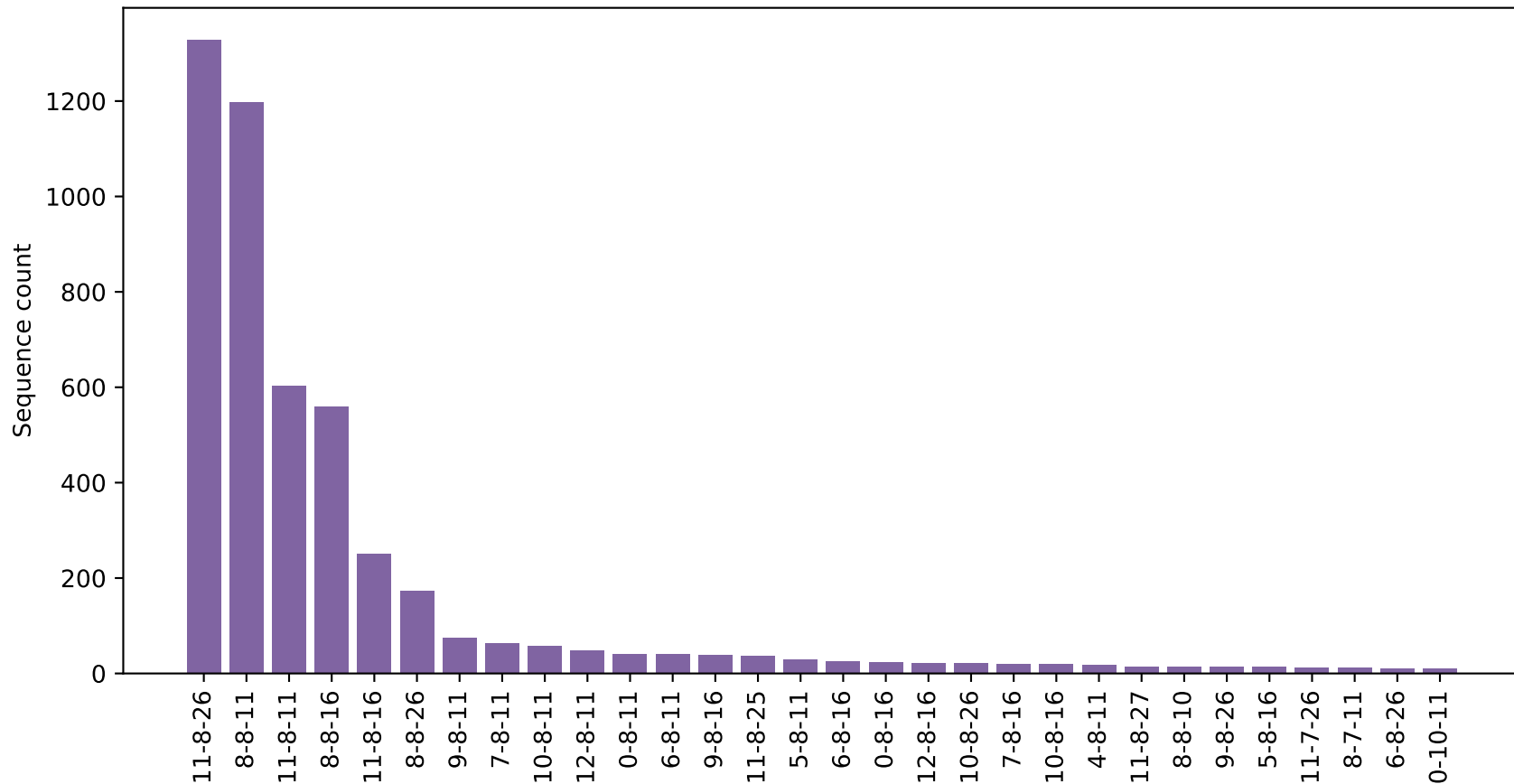
Top 30 CDR1-CDR2-CDR3 length combinations
