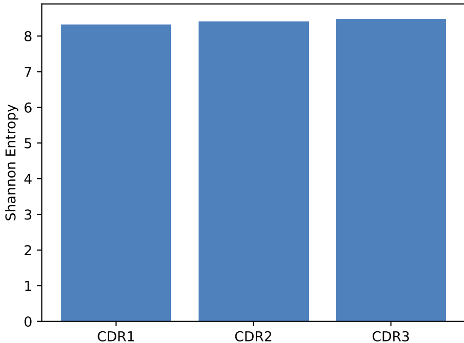
CDR Shannon entropy
