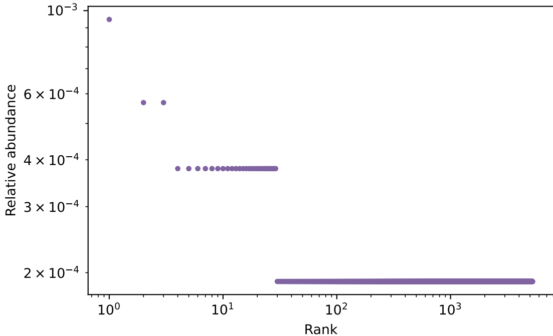
Clonal abundance rank curve
