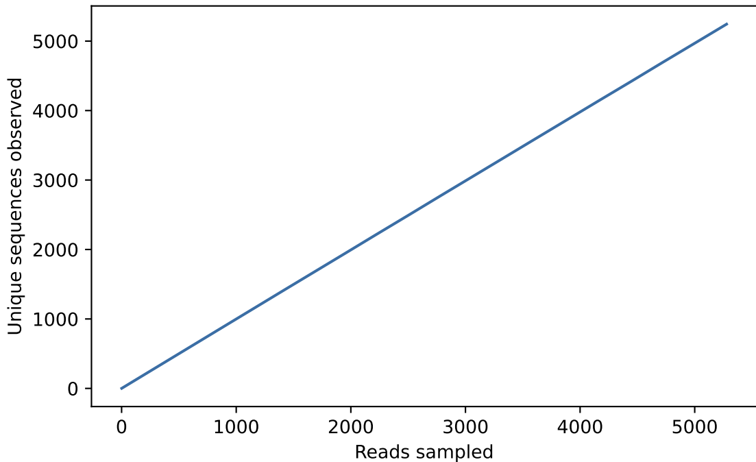
Rarefaction: unique AA sequences vs read depth
