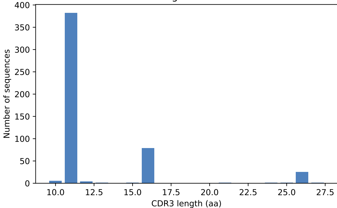
CDR3 length distribution
