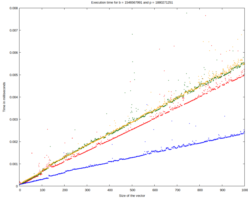
Figure 5: Execution time comparison between the two versions of multiply low
