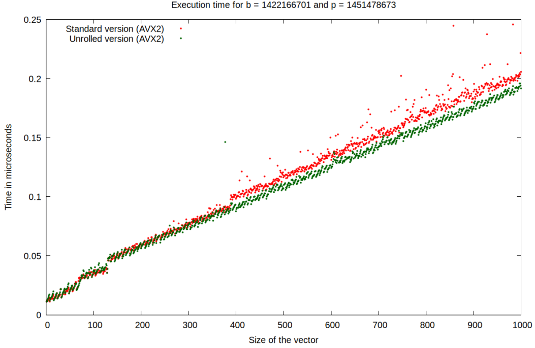
Figure 1: Execution time (in microseconds) comparison: Standard vs. Unrolled
