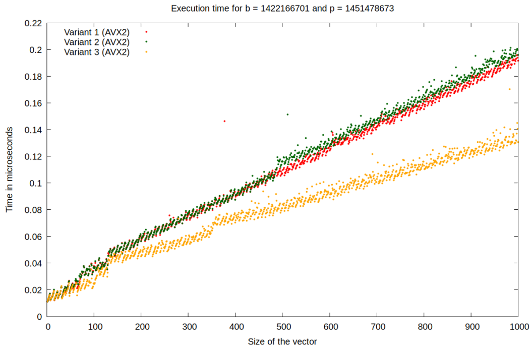
Figure 2: Execution time (in microseconds) comparison of all implementation variants
