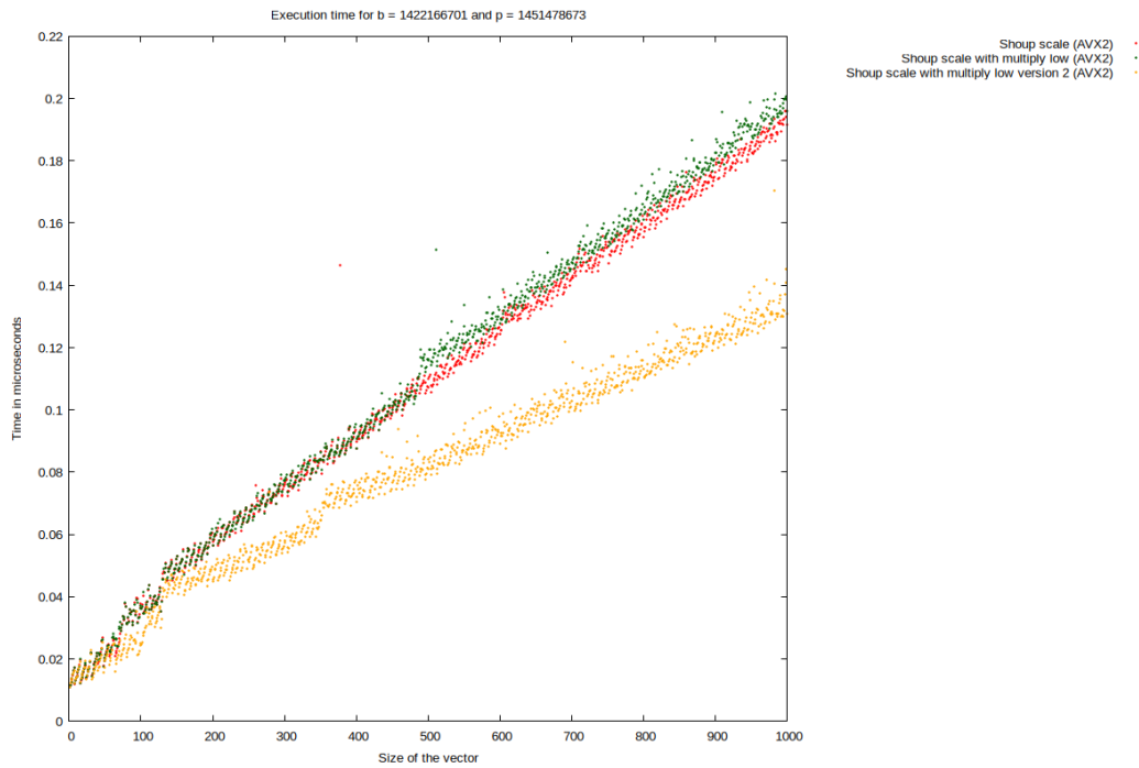
Figure 2: Execution time (in microseconds) comparison of all implementation variants
