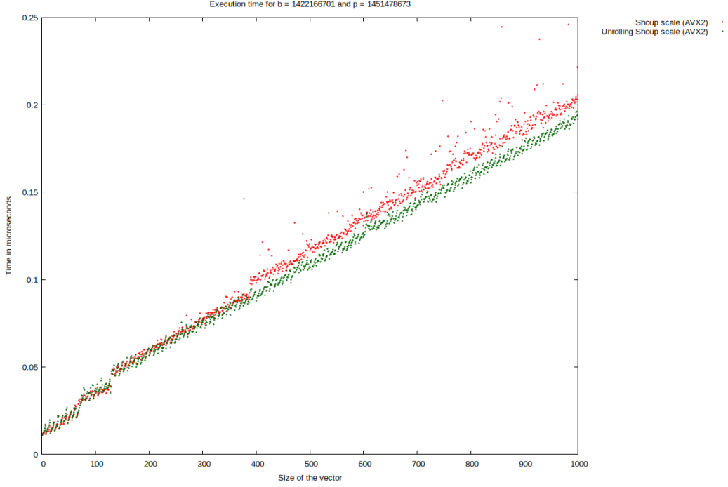
Figure 1: Execution time (in microseconds) comparison: Standard vs. Unrolled
