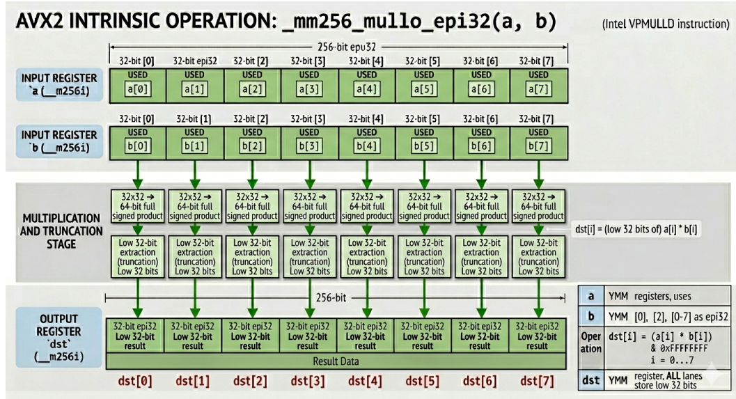
Figure 7: Diagram of mullo_epi32 for AVX2 (Gemini)
