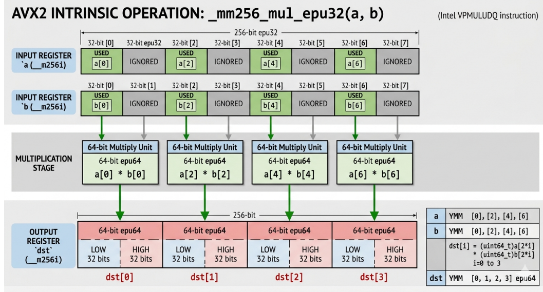
Figure 6: Diagram of mul_epu32 for AVX2 (Gemini)
