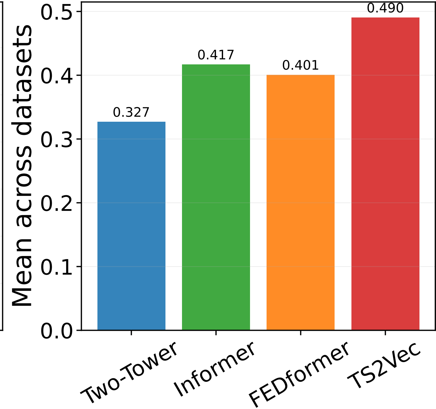
LOSS
