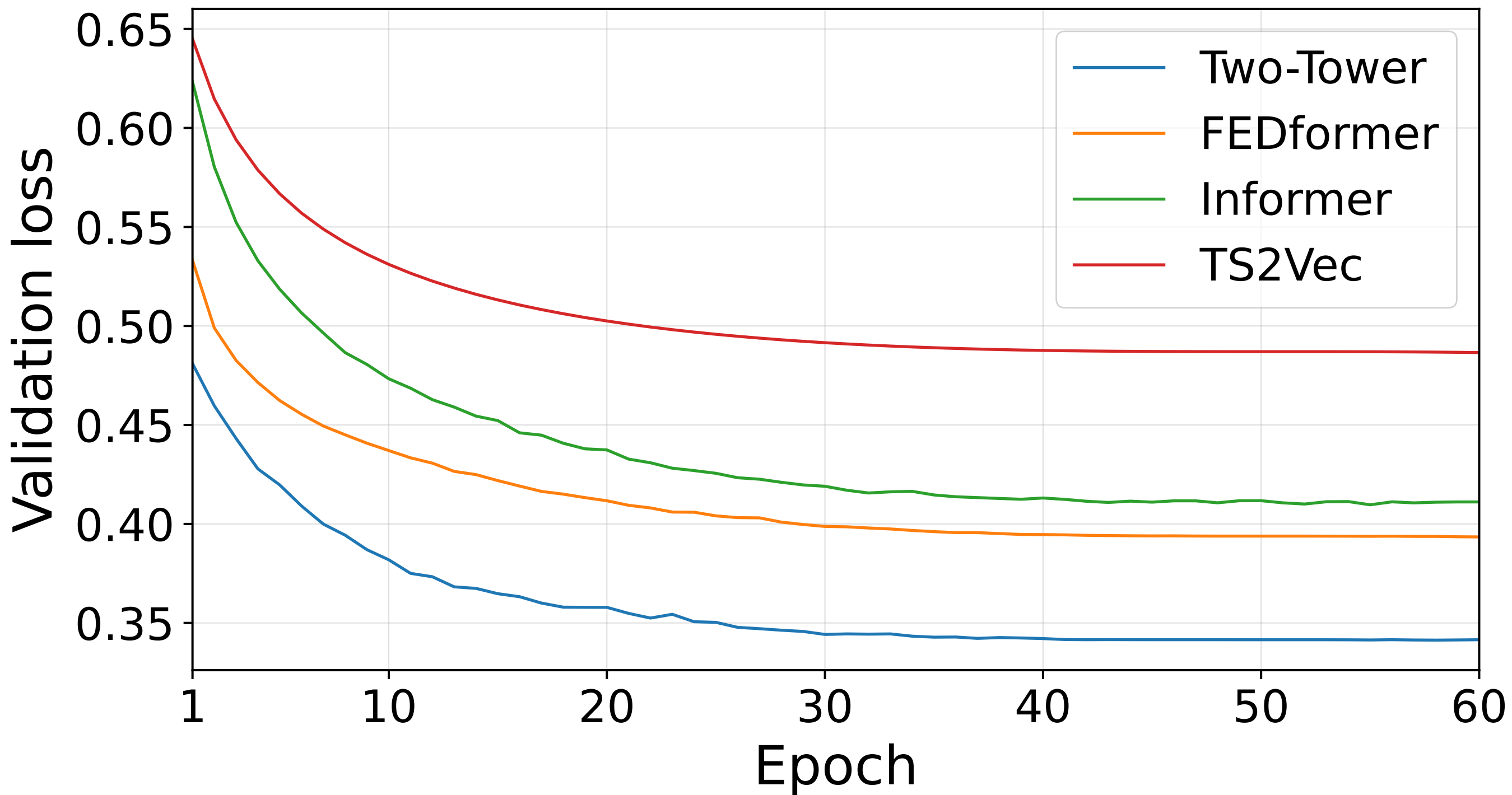
Mean validation loss across 124 common UCR datasets
