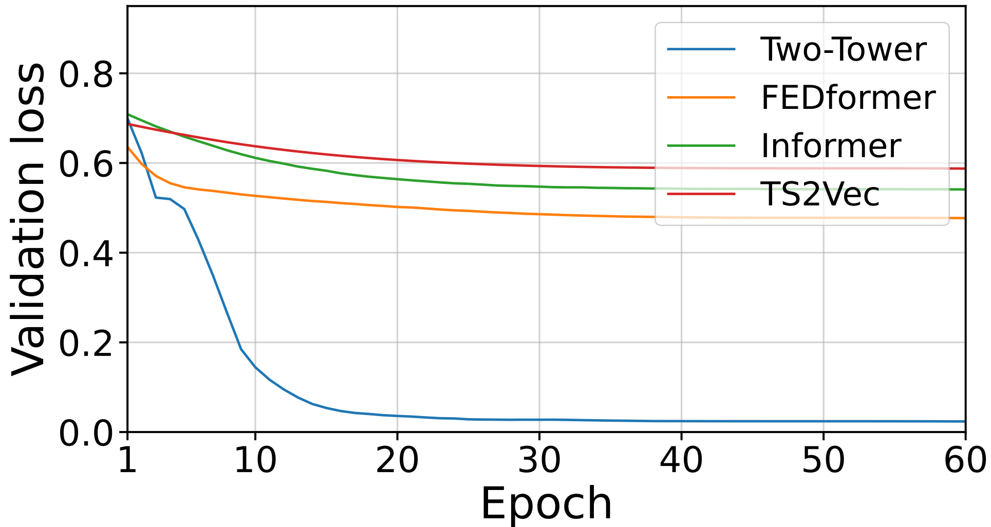
CinCECGTorso — Validation Loss
