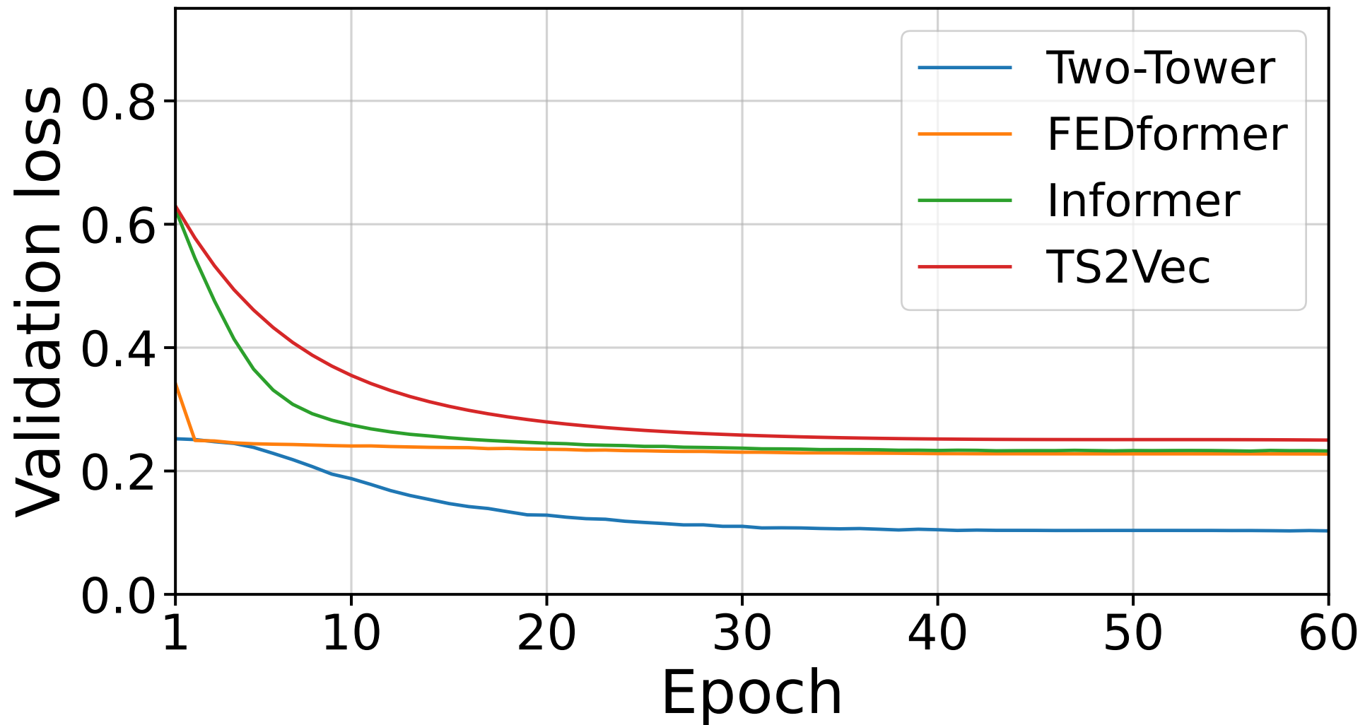
FacesUCR — Validation Loss
