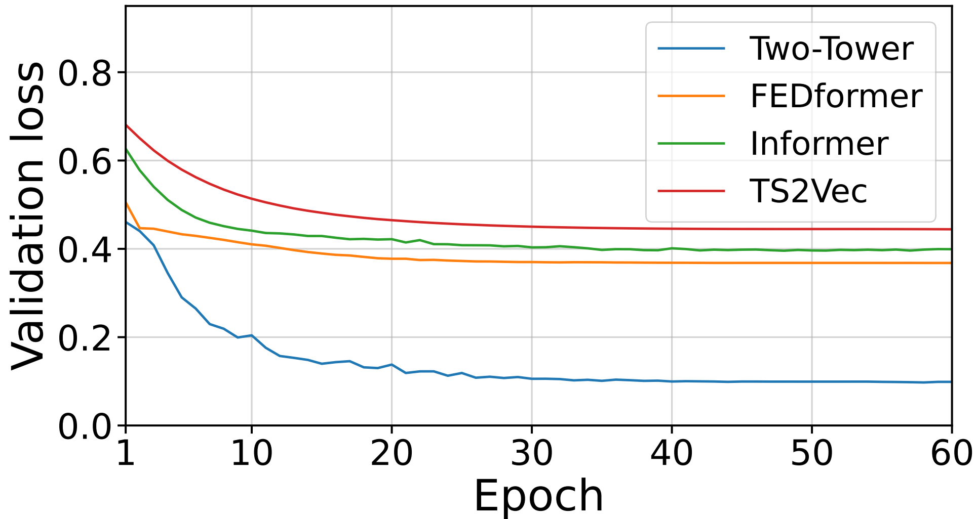
GesturePebbleZ1 — Validation Loss
