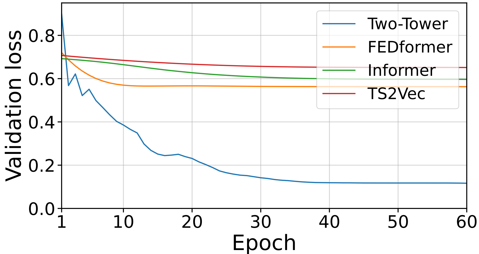
Rock — Validation Loss
